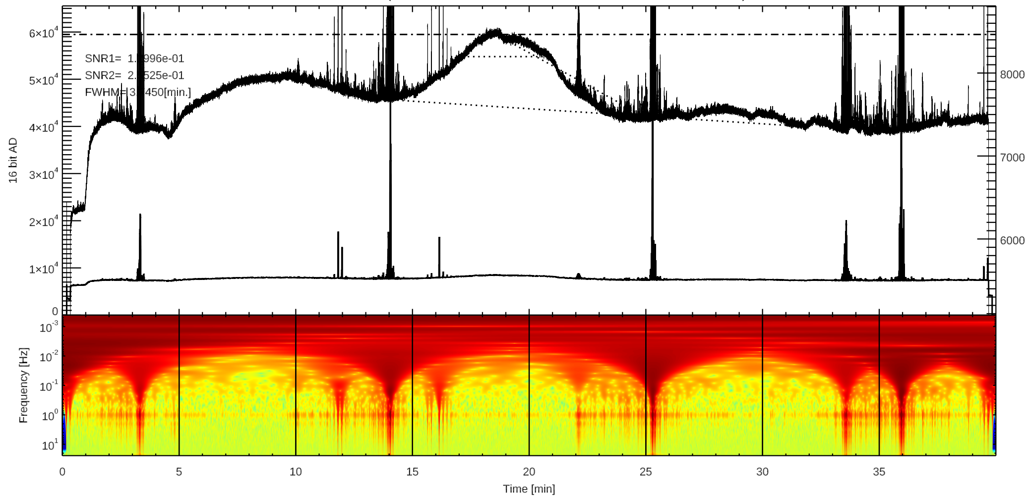
C 3C157 (/home4/archive/swift/dat/2026/01/T20260105224925.dat)
