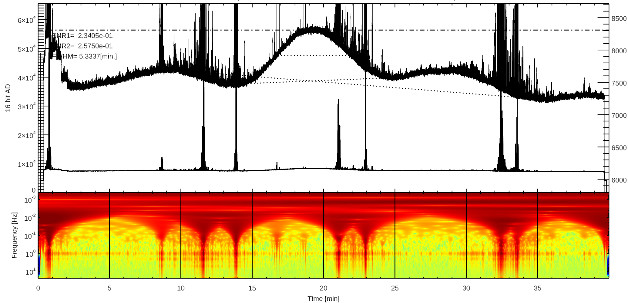
C 3C157 (/home4/archive/swift/dat/2026/01/T20260106224530.dat)
