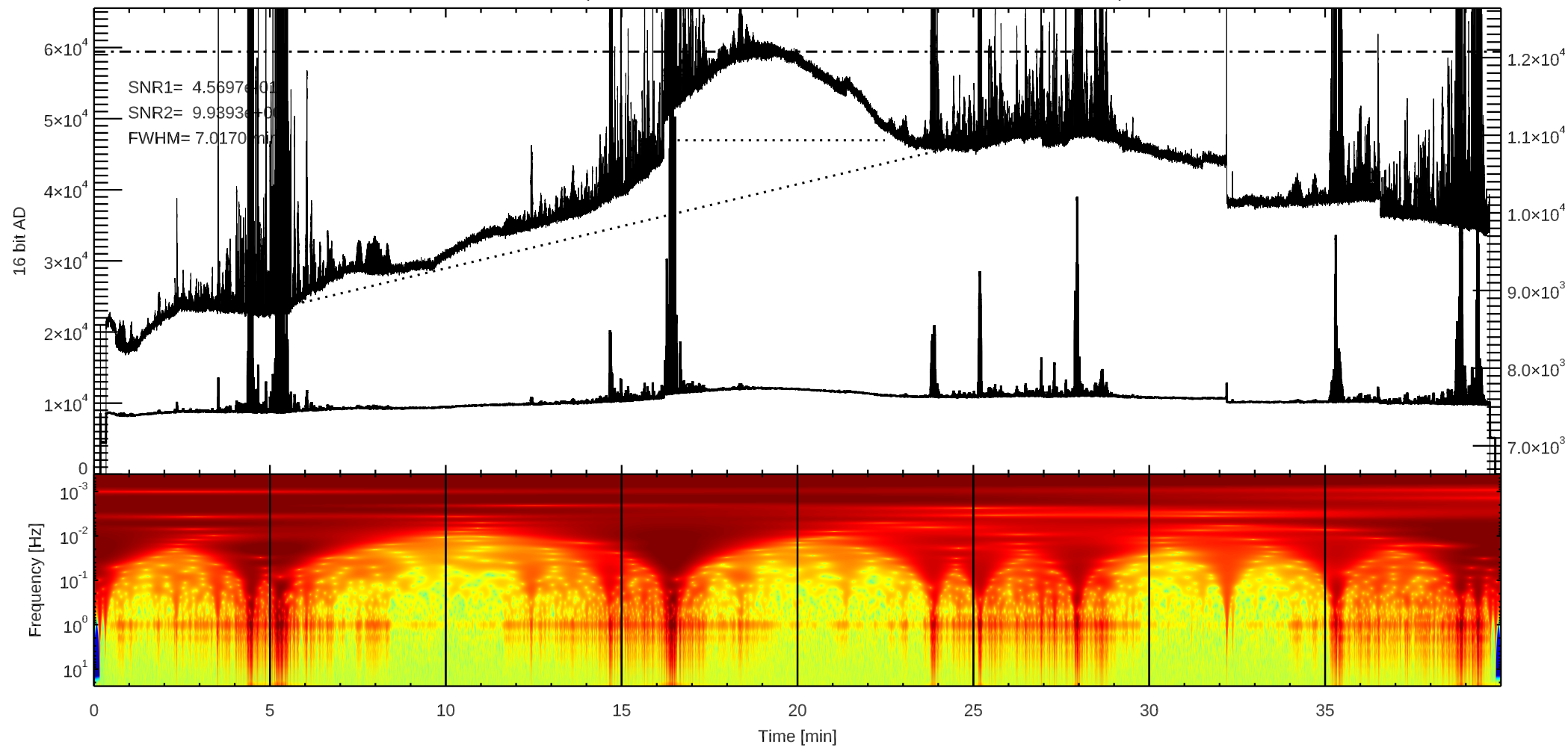
C 3C157 (/home4/archive/swift/dat/2026/01/T20260109223342.dat)
