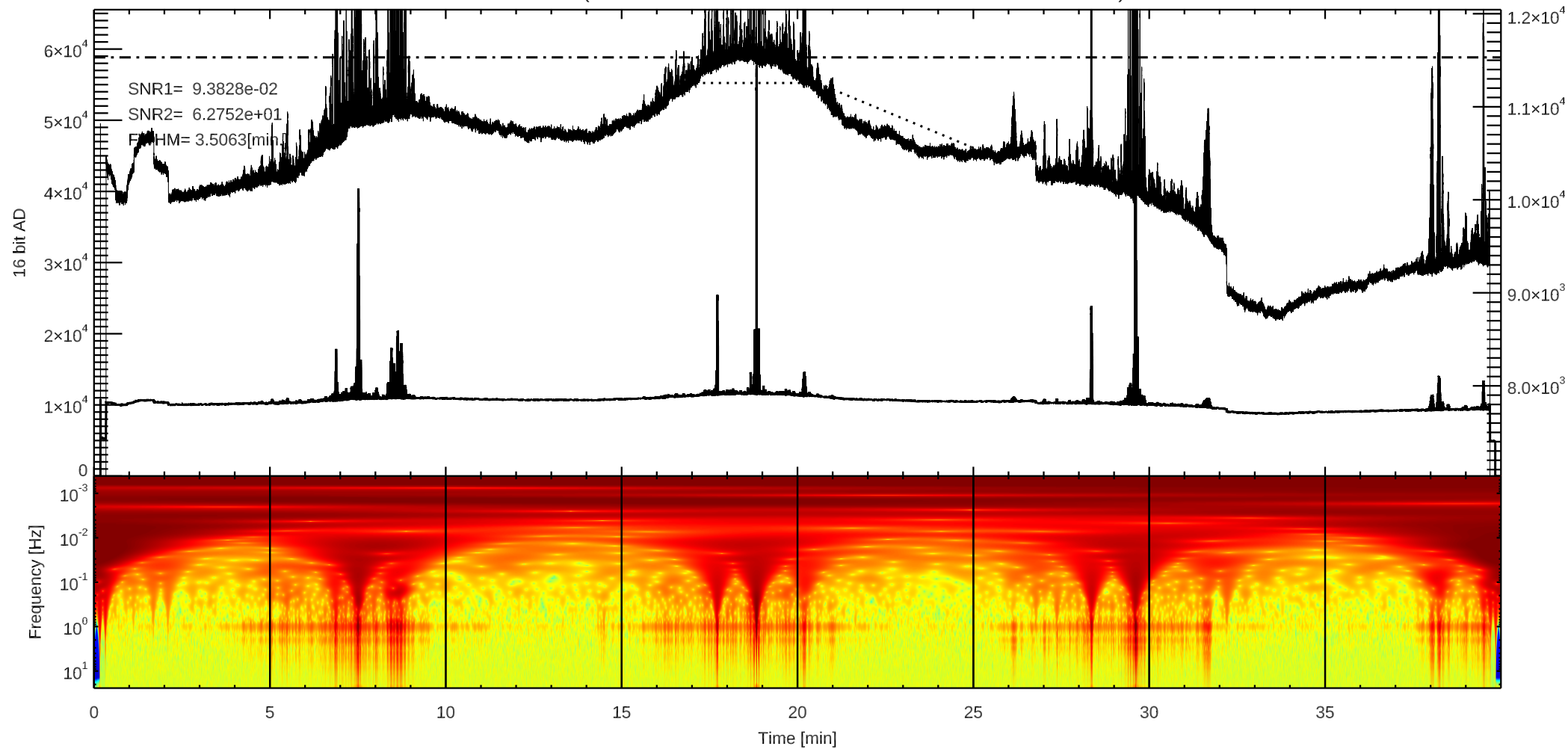
C 3C157 (/home4/archive/swift/dat/2026/01/T20260114221402.dat)
