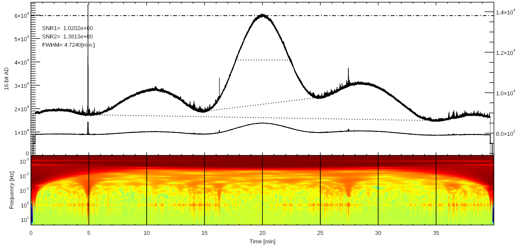
C 3C274 (/home4/archive/swift/dat/2026/01/T20260107045700.dat)
