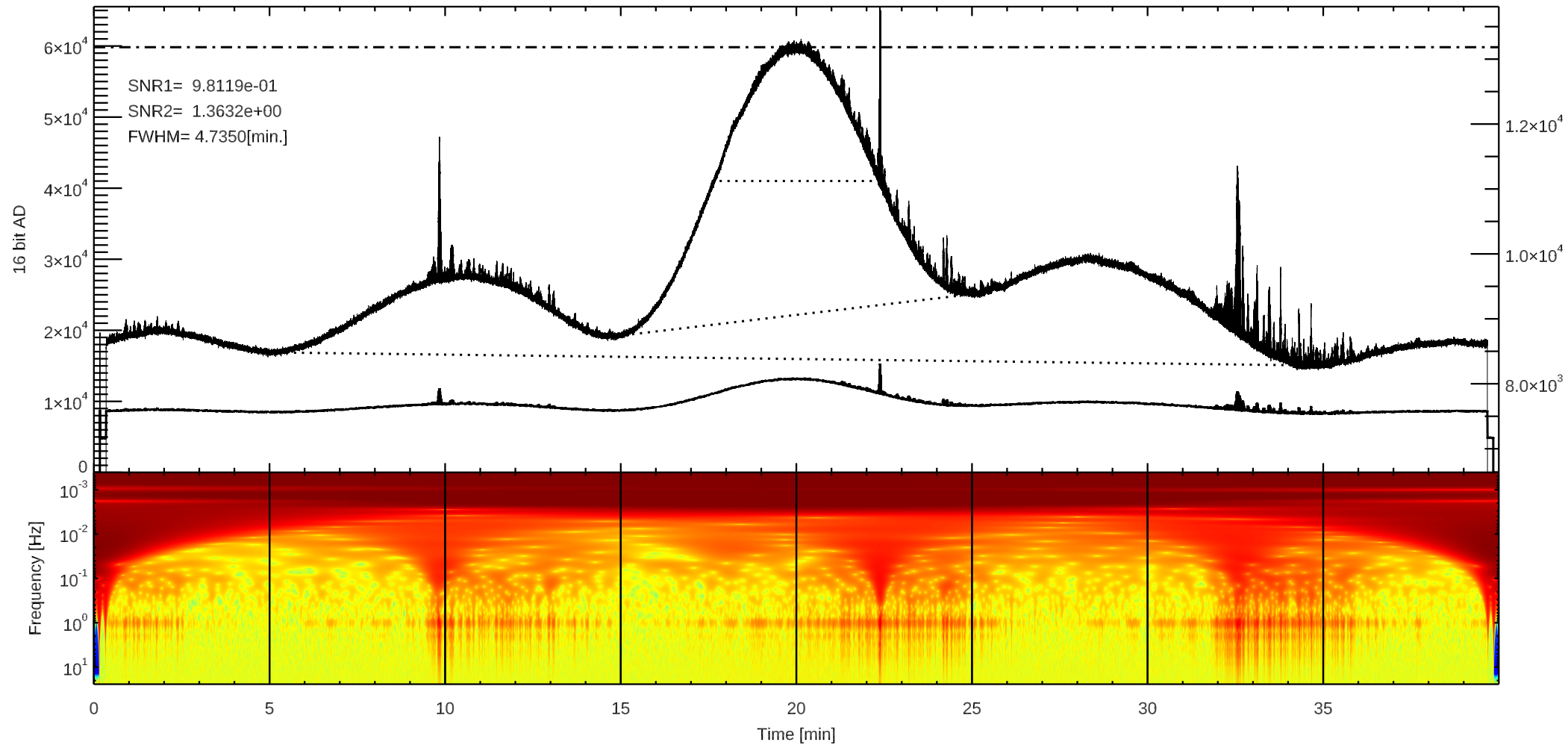
C 3C274 (/home4/archive/swift/dat/2026/01/T20260109044909.dat)
