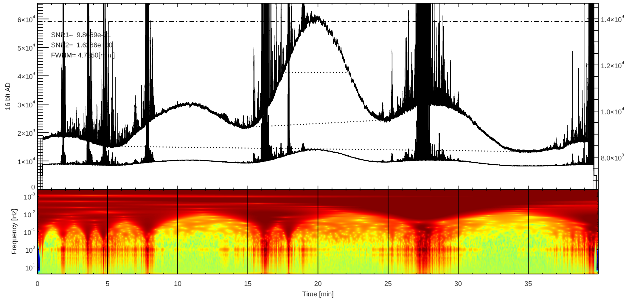
C 3C274 (/home4/archive/swift/dat/2026/01/T20260112043721.dat)
