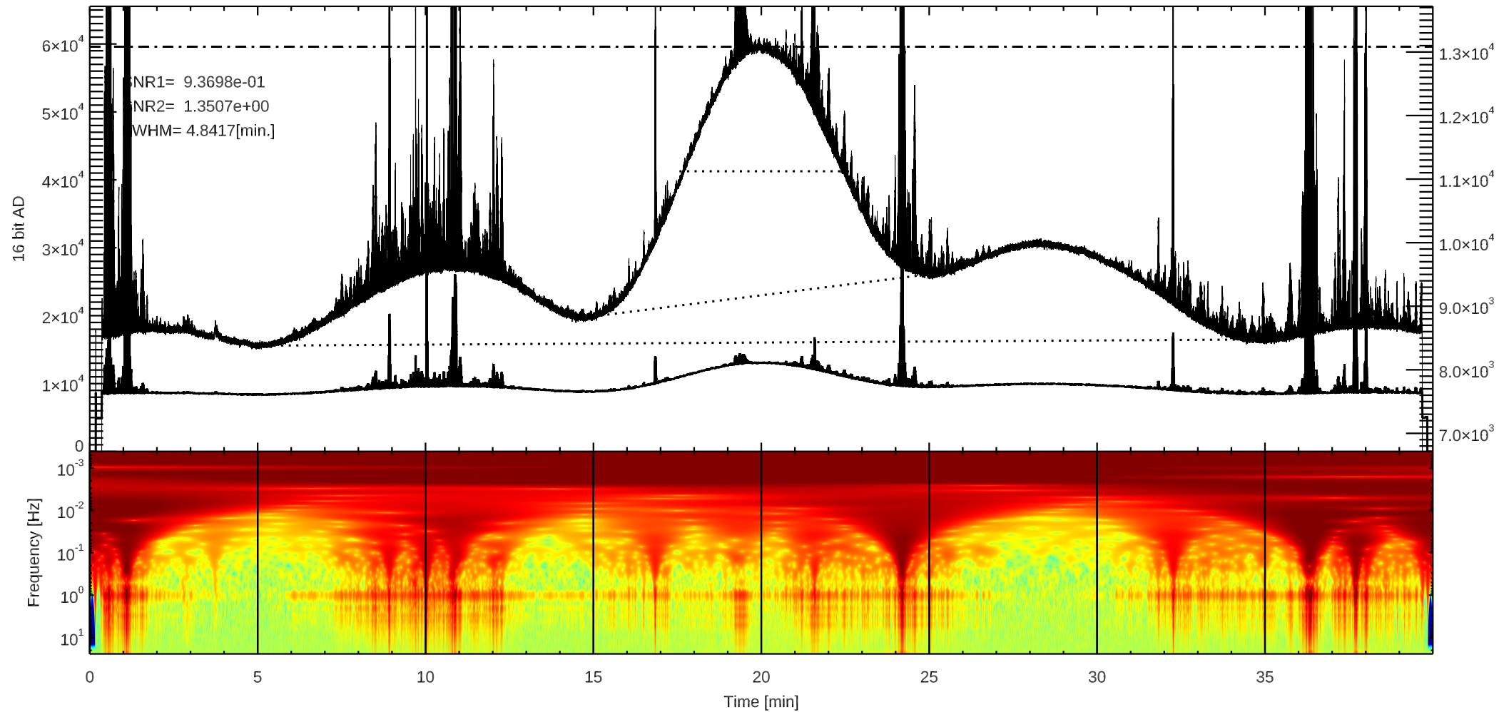
C 3C274 (/home4/archive/swift/dat/2026/01/T20260115042533.dat)
