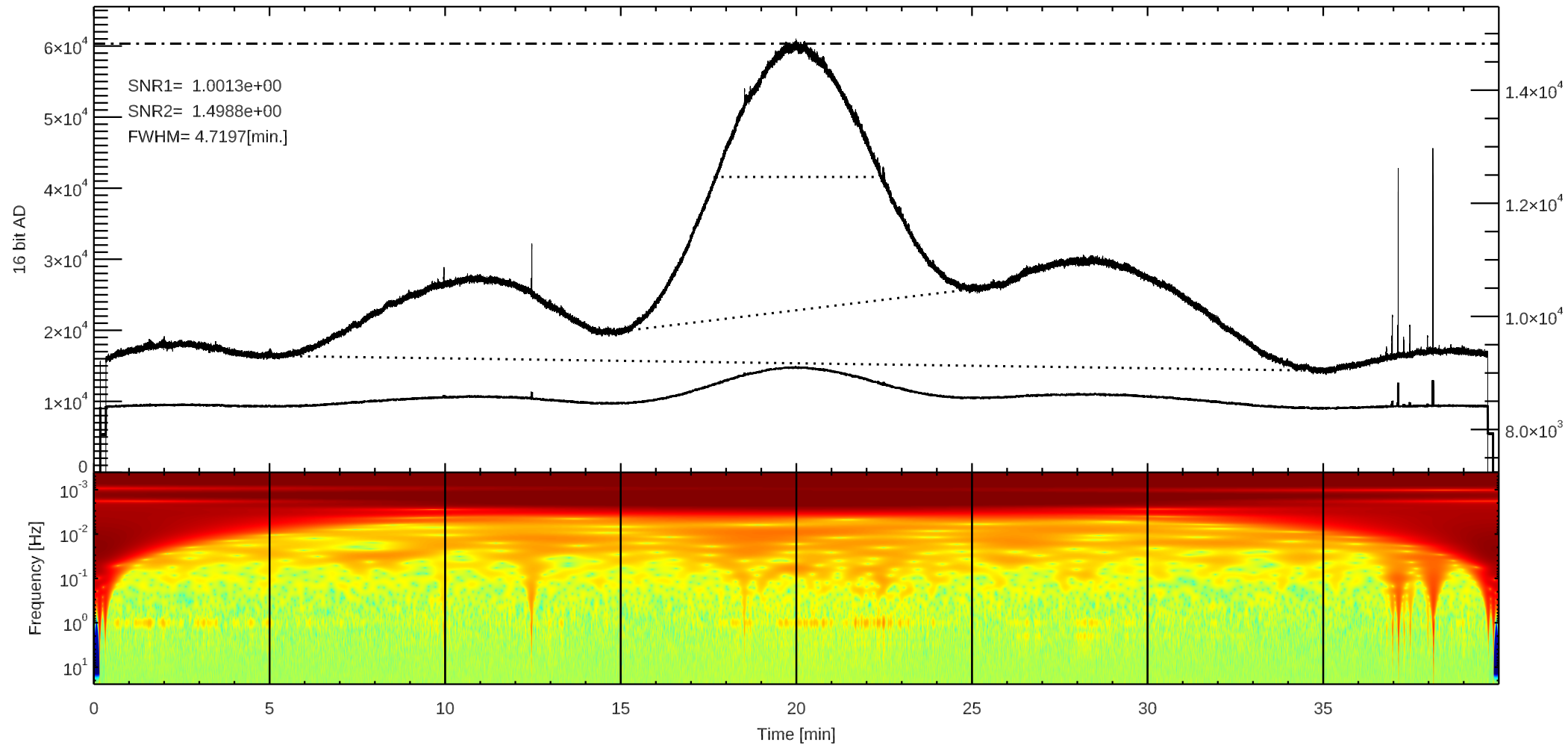
C 3C274 (/home4/archive/swift/dat/2026/01/T20260130032635.dat)
