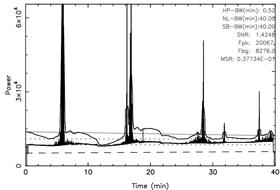
TOYOKAWA 3C123 2026/01/14(014)20:33:24-21:13:24JST
