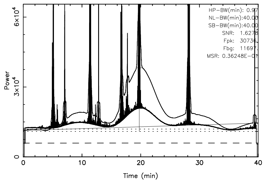
TOYOKAWA 3C144 2026/01/14(014)21:30:36-22:10:36JST
