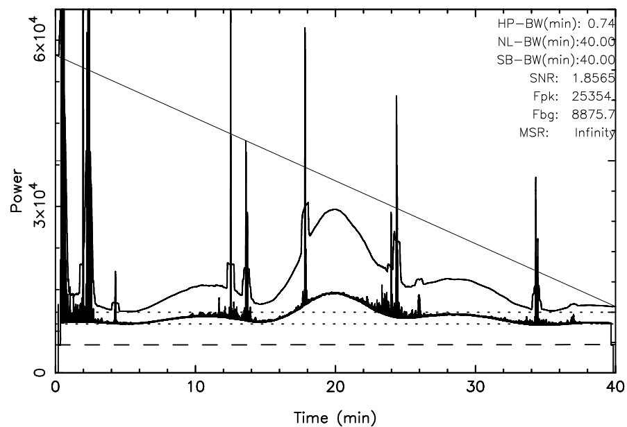
TOYOKAWA 3C274 2026/01/14(014)04:29:27-05:09:27JST
