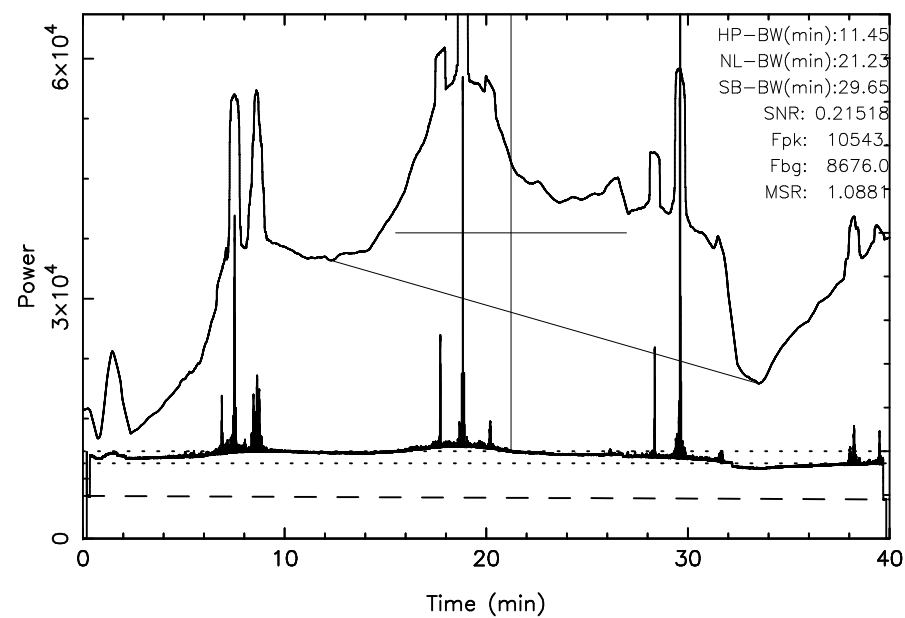
TOYOKAWA 3C157 2026/01/14(014)22:14:00-22:54:00JST
