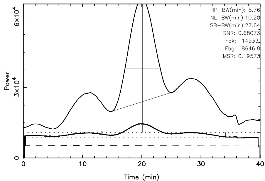
TOYOKAWA 3C274 2026/01/29(029)03:30:28-04:10:28JST
