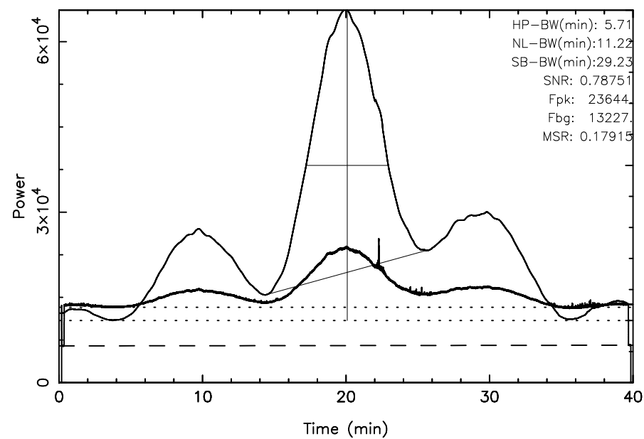
TOYOKAWA 3C144 2026/01/29(029)20:31:38-21:11:38JST
