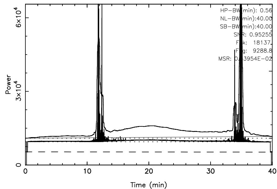
TOYOKAWA 3C295 2026/01/29(029)05:10:19-05:50:19JST
