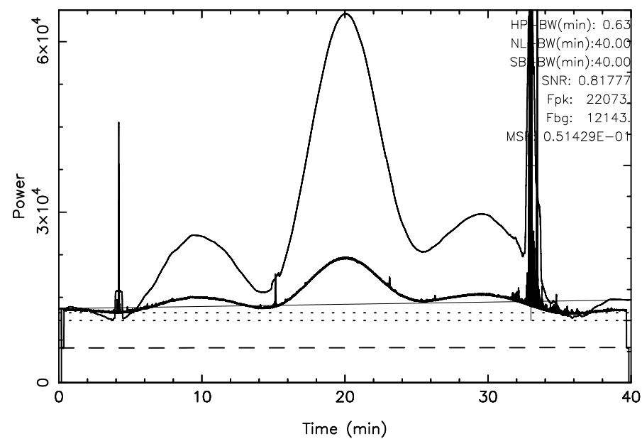
TOYOKAWA 3C144 2026/02/07(038)19:56:14-20:36:14JST
