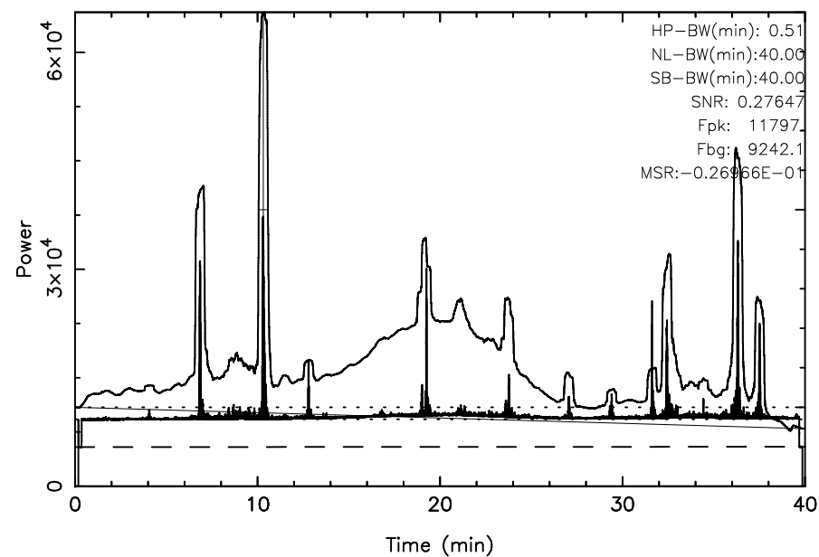
TOYOKAWA 3C295 2026/02/07(038)04:34:56-05:14:56JST
