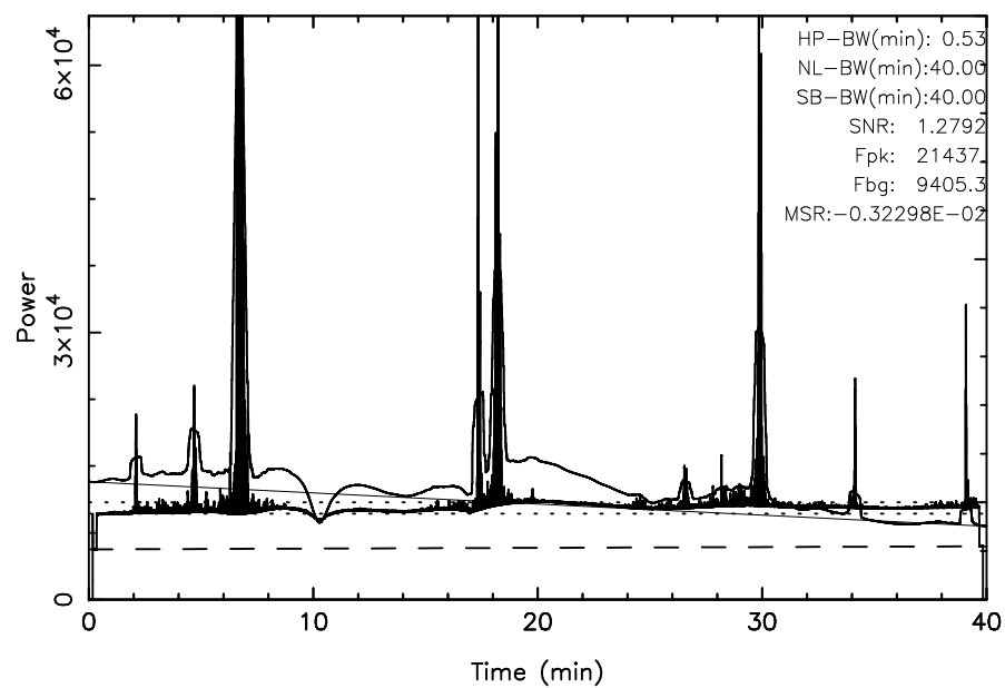
TOYOKAWA 3C123 2026/02/07(038)18:59:02-19:39:02JST
