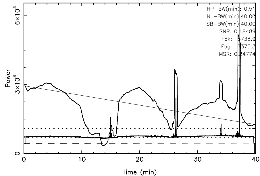
TOYOKAWA 3C295 2026/03/21(080)01:49:48-02:29:48JST
