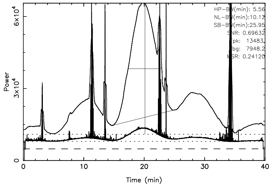
TOYOKAWA 3C274 2026/03/21(080)00:09:58-00:49:58JST
