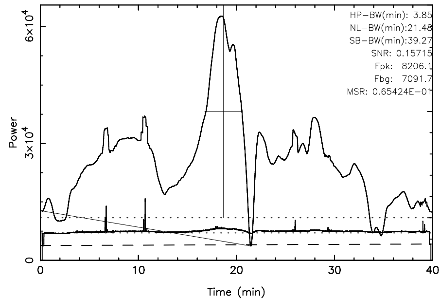
TOYOKAWA 3C157 2026/03/21(080)17:54:31-18:34:31JST
