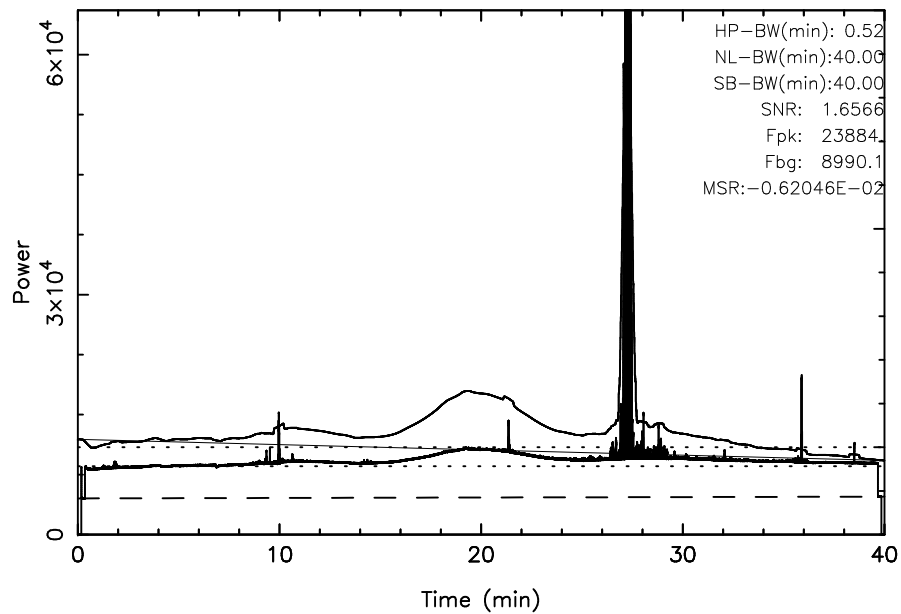
TOYOKAWA 3C348 2026/03/21(080)04:29:32-05:09:32JST
