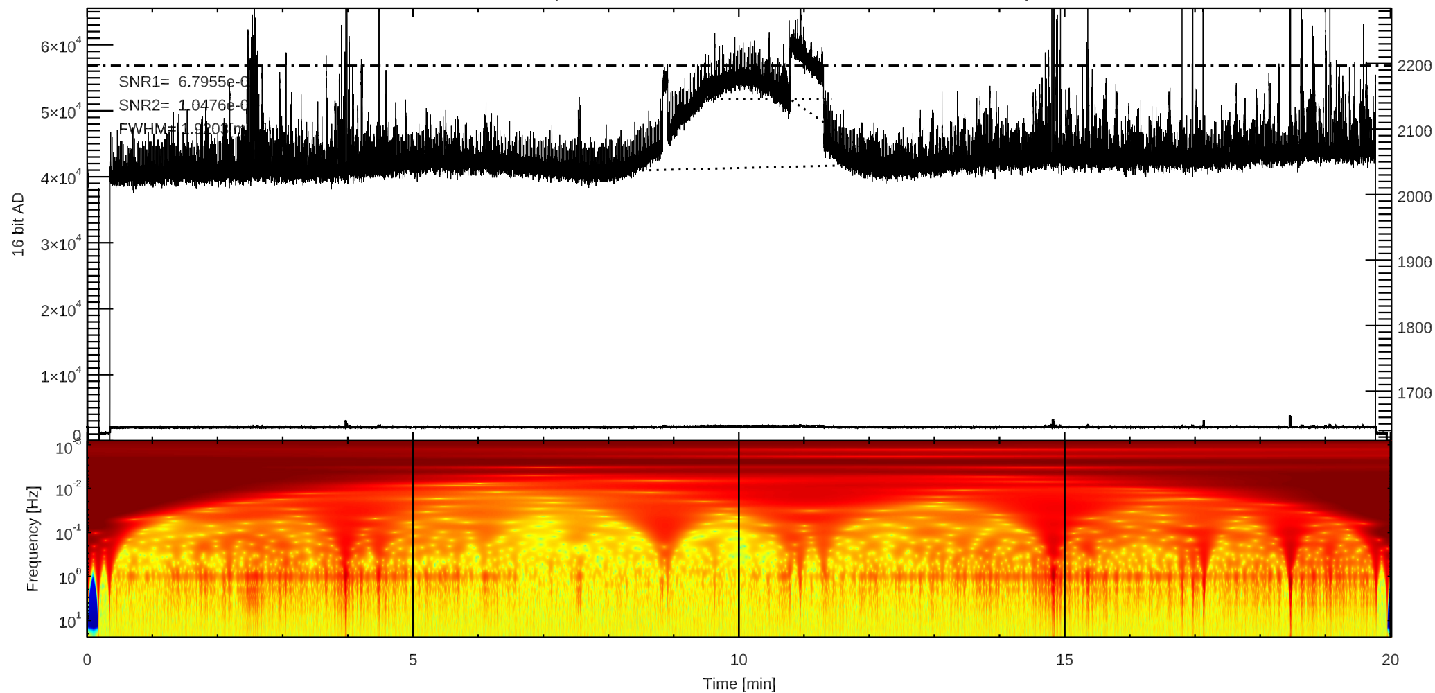
C 3C348 (/home4/archive/fit/dat/2026/07/F20260711211516.dat)
