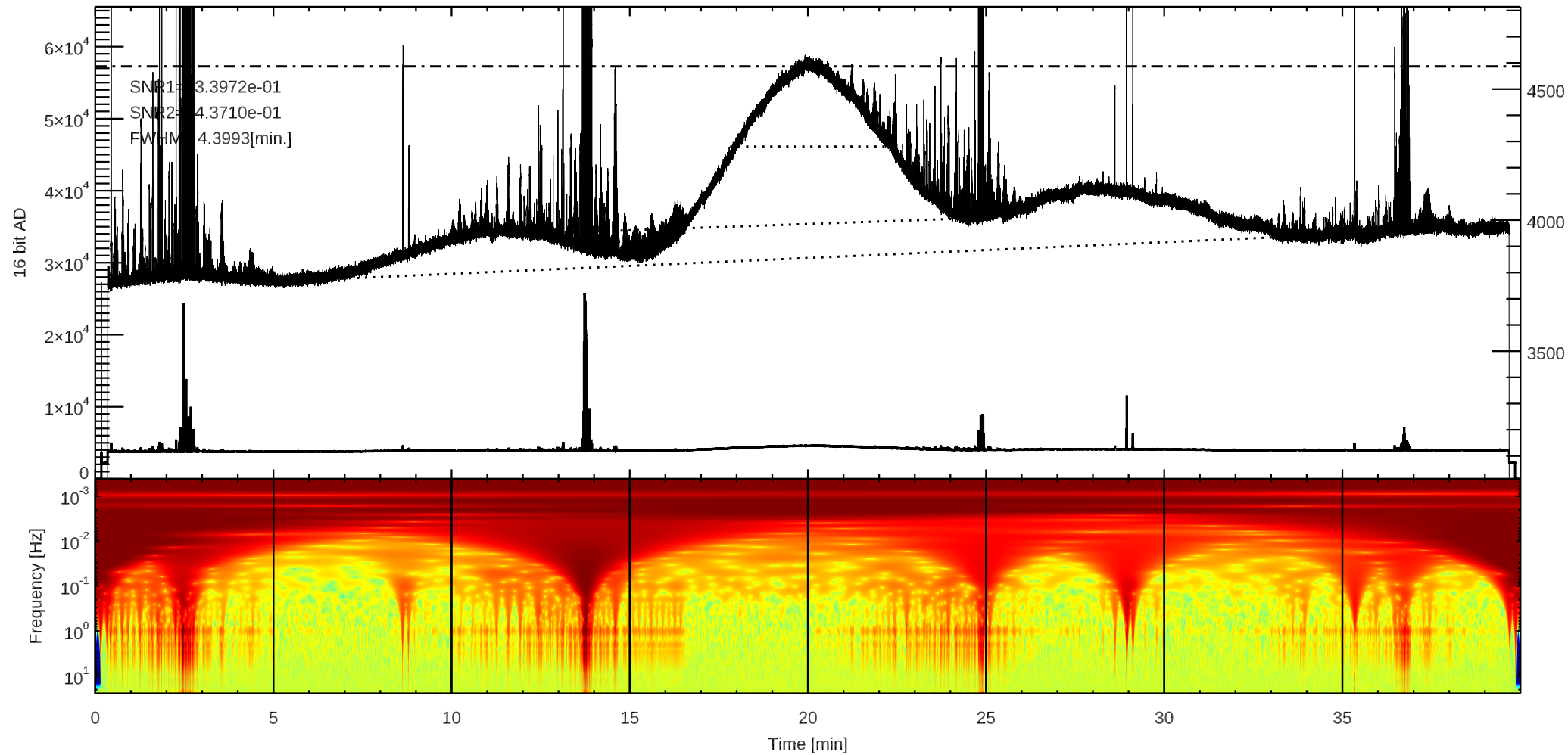
C 3C348 (/home4/archive/swift/dat/2026/07/T20260718203746.dat)
