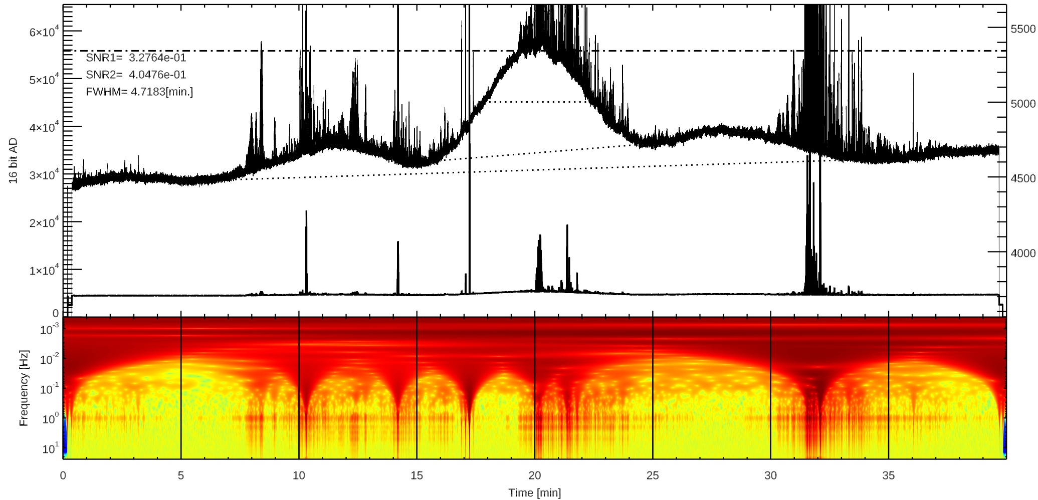
C 3C348 (/home4/archive/swift/dat/2026/07/T20260724201411.dat)
