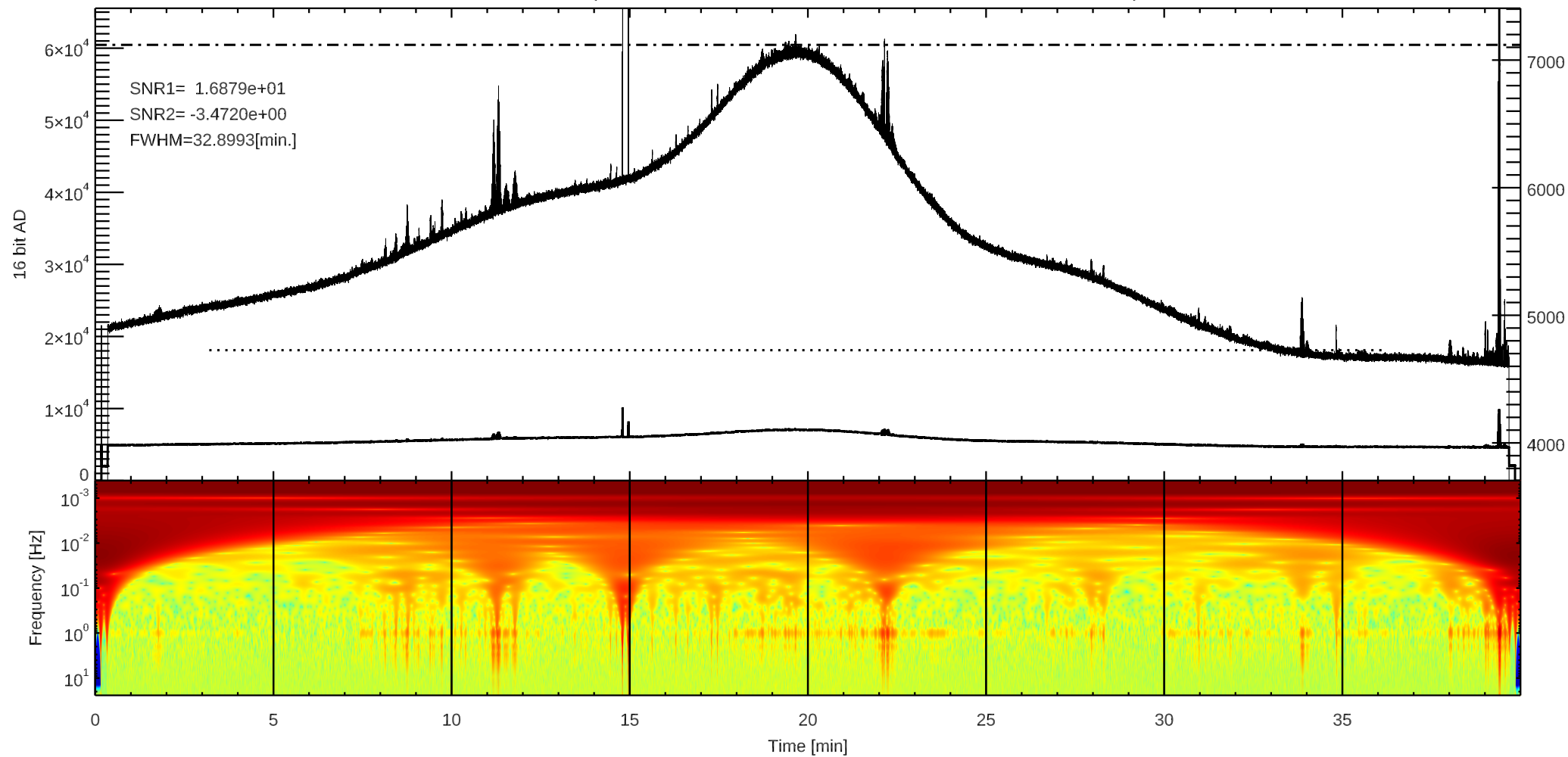
C 3C392 (/home4/archive/swift/dat/2026/07/T20260713230205.dat)
