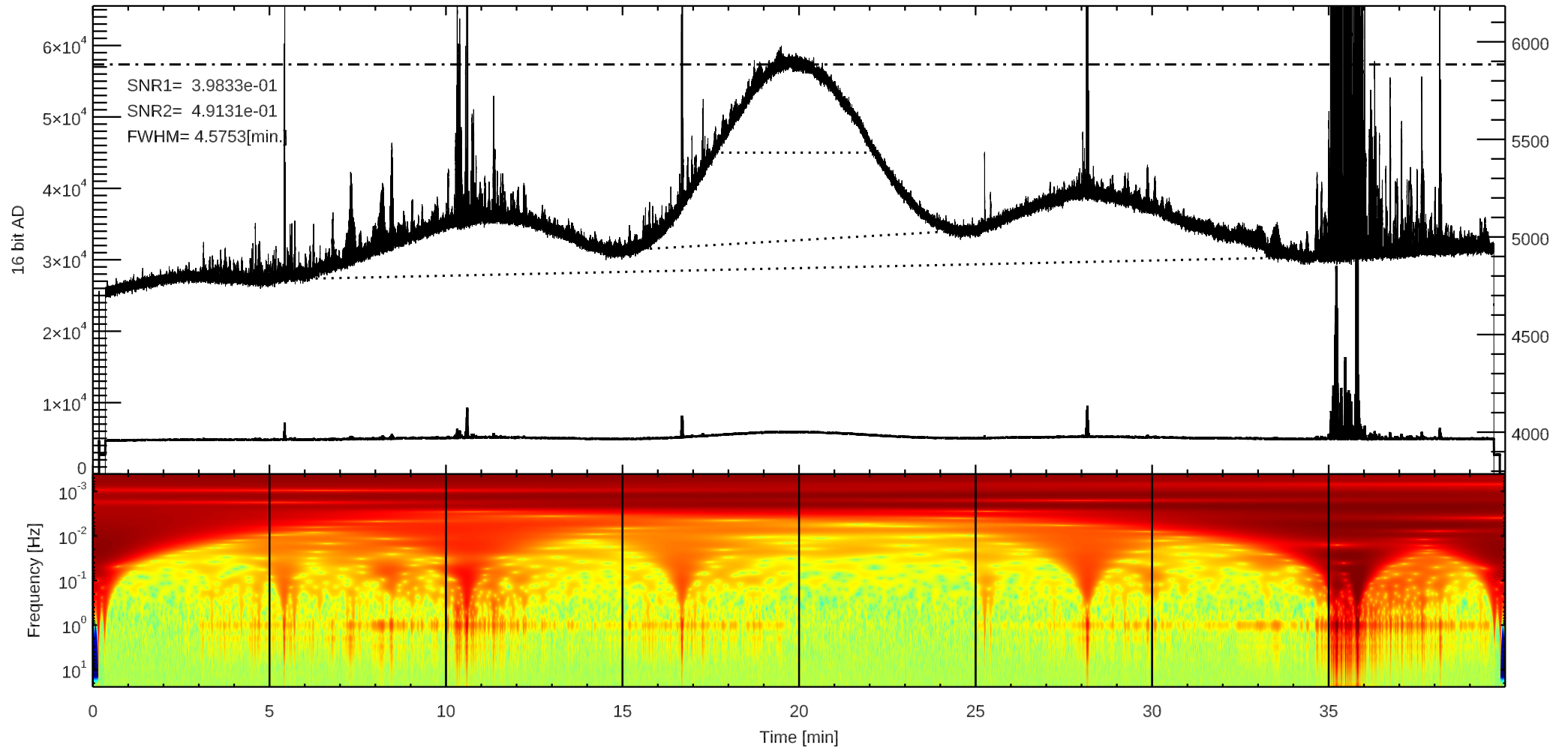
C 3C348 (/home4/archive/swift/dat/2026/08/T20260812185929.dat)
