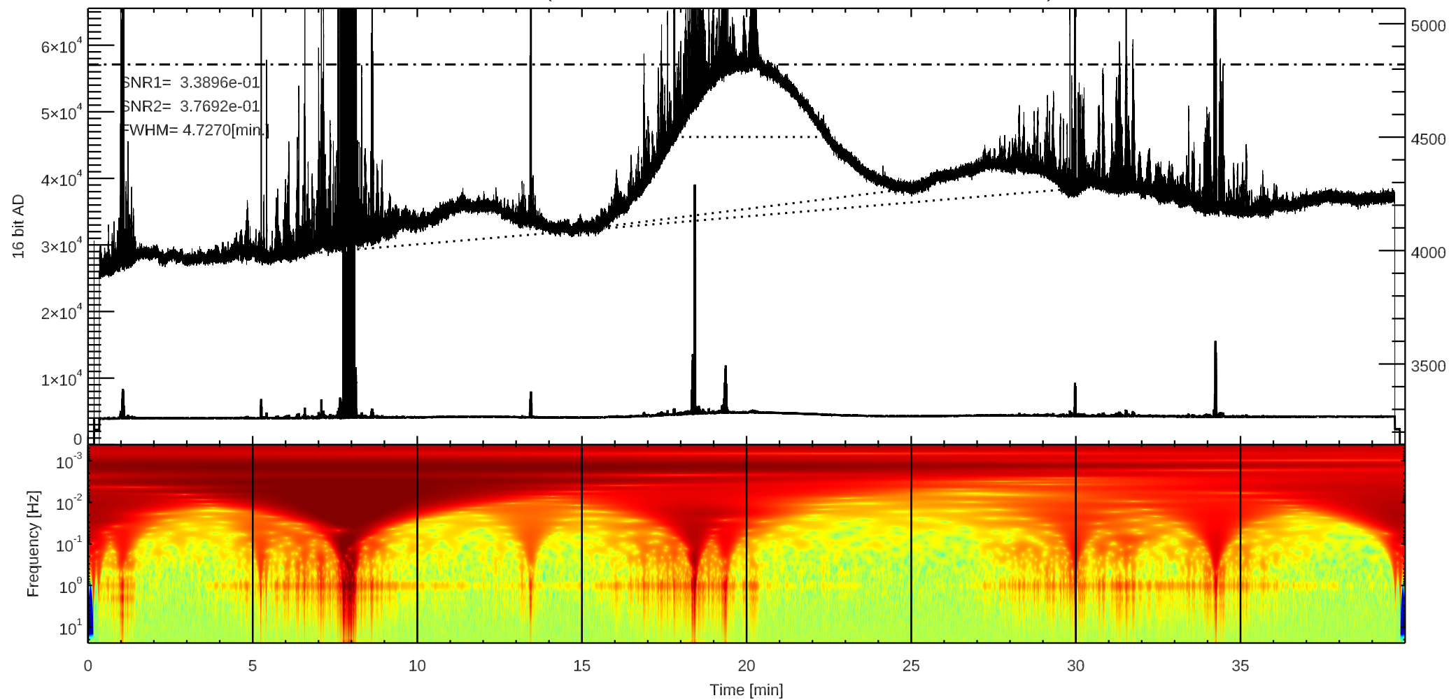
C 3C348 (/home4/archive/swift/dat/2026/08/T20260820182801.dat)
