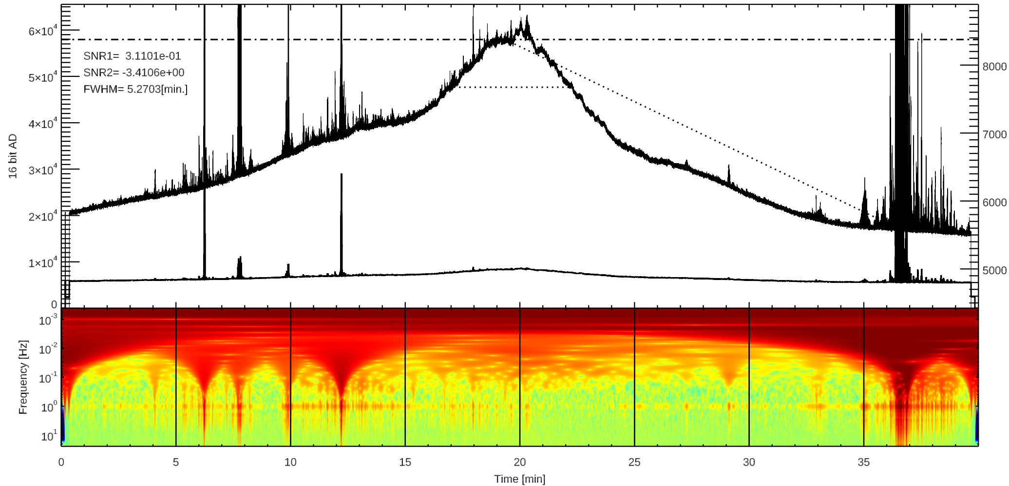
C 3C392 (/home4/archive/swift/dat/2026/08/T20260805213139.dat)
