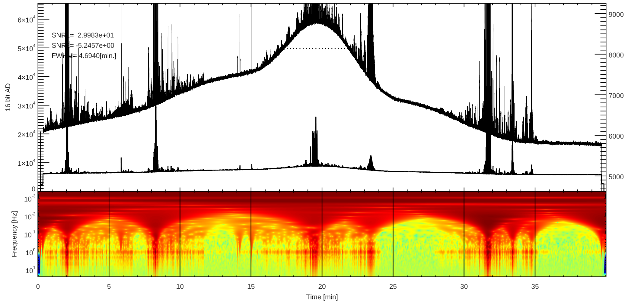
C 3C392 (/home4/archive/swift/dat/2026/08/T20260811210803.dat)
