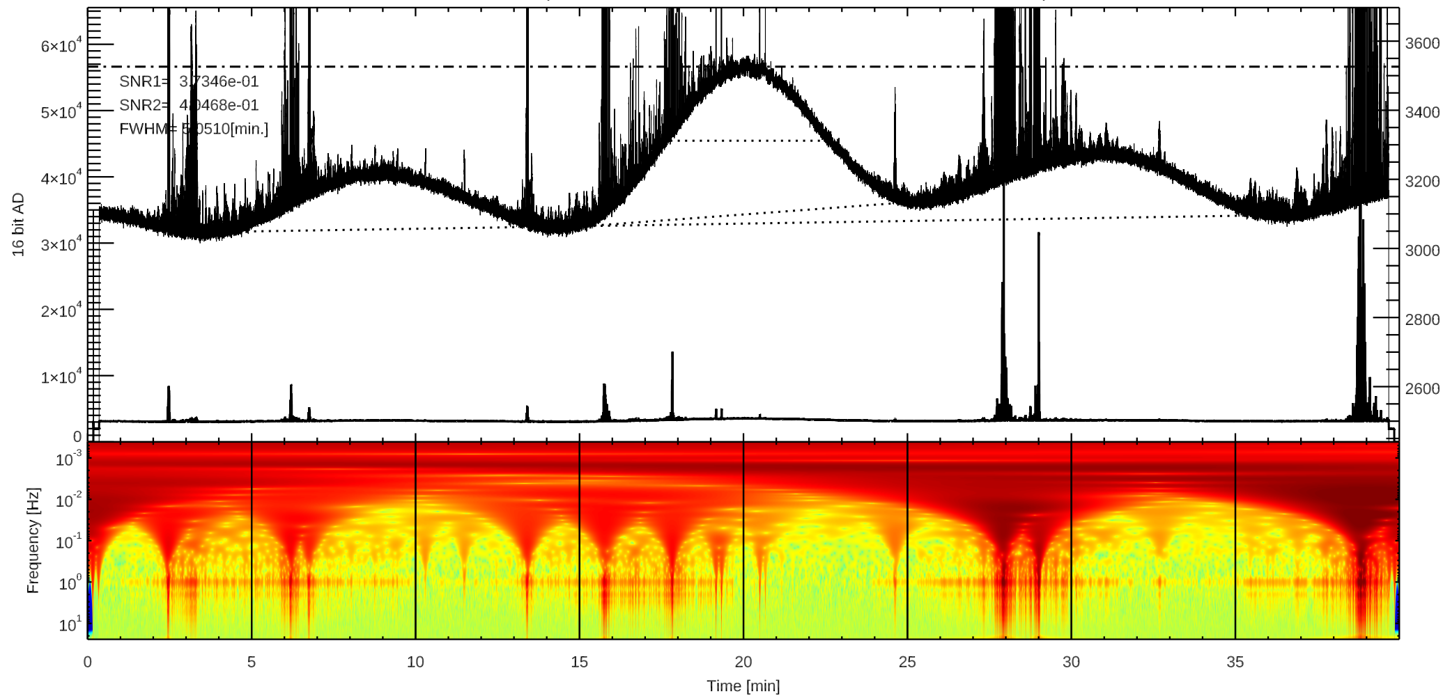
C 3C123 (/home4/archive/swift/dat/2026/09/T20260912044551.dat)
