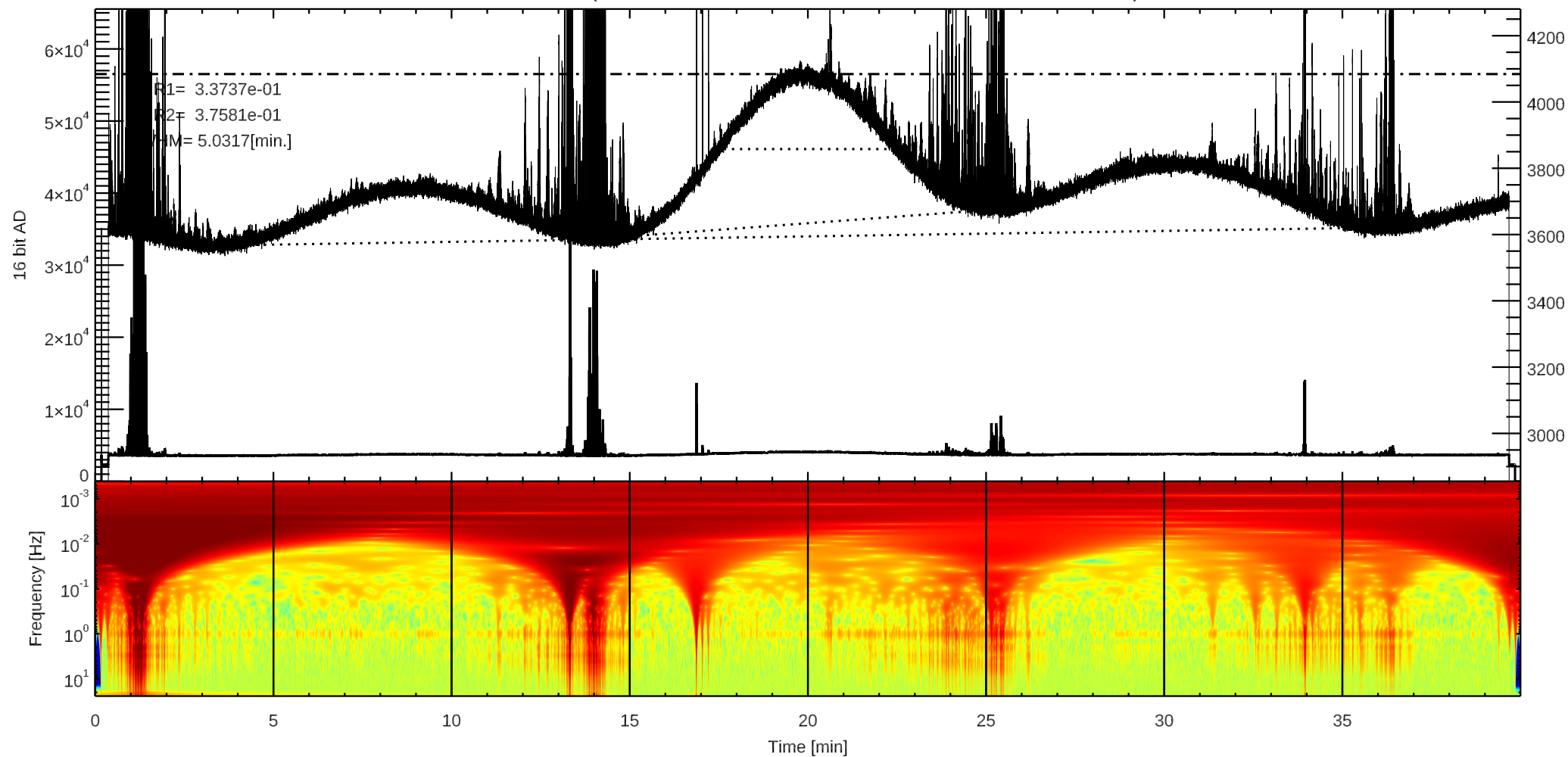
C 3C123 (/home4/archive/swift/dat/2026/09/T20260919041820.dat)
