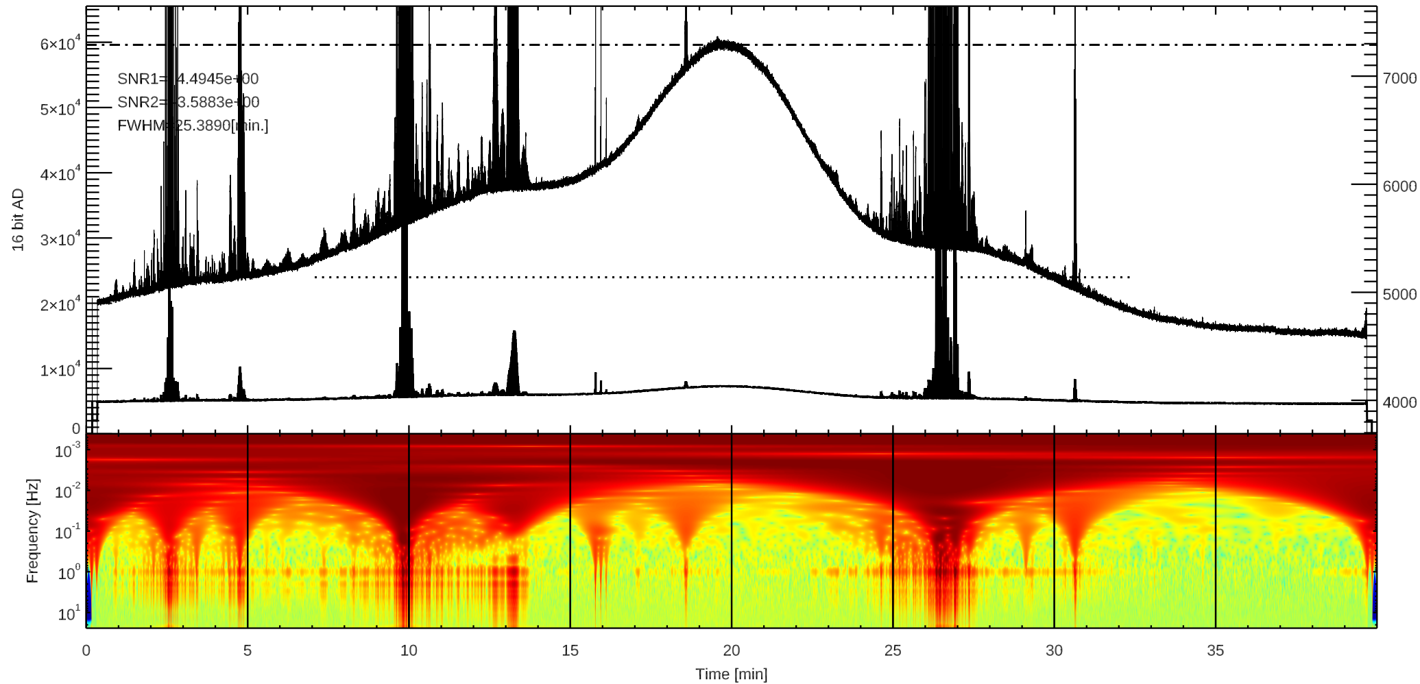
C 3C392 (/home4/archive/swift/dat/2026/09/T20260910191003.dat)
