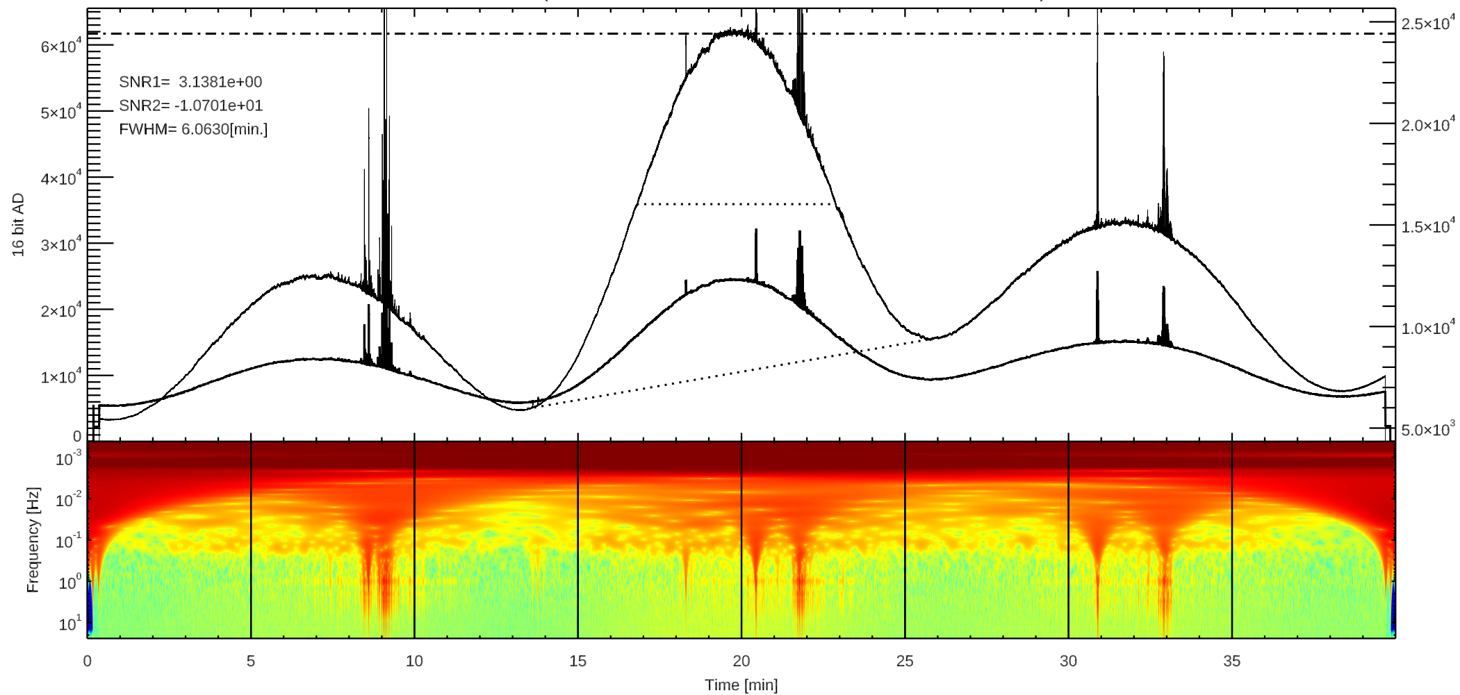
C 3C405 (/home4/archive/swift/dat/2026/09/T20260923192144.dat)
