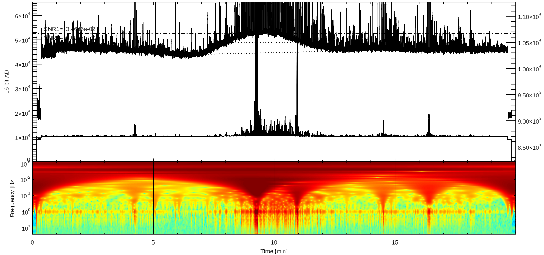
C 3C123 (/home4/archive/kit/dat/2026/10/K20261018023421.dat)
