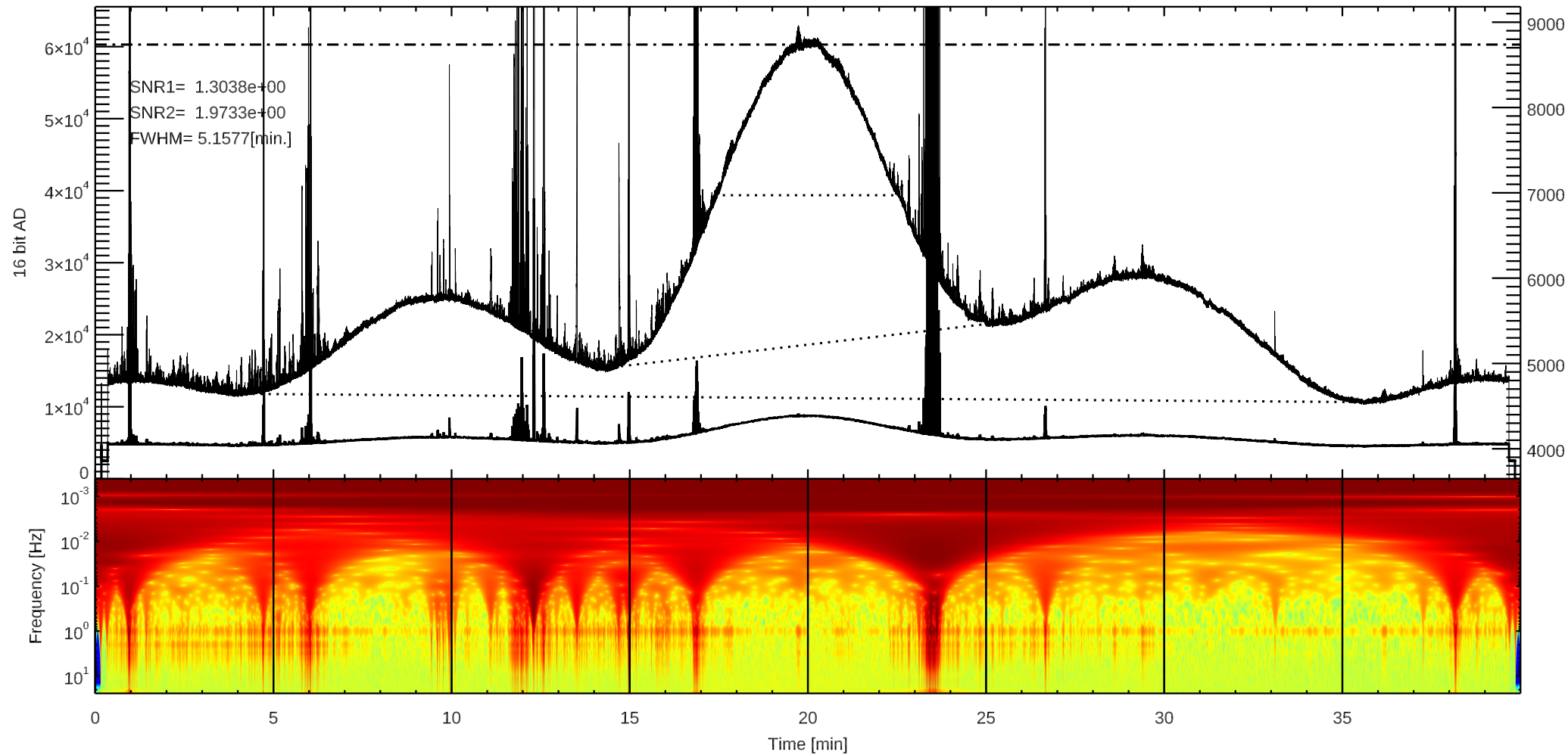
C 3C144 (/home4/archive/swift/dat/2026/10/T20261006040843.dat)
