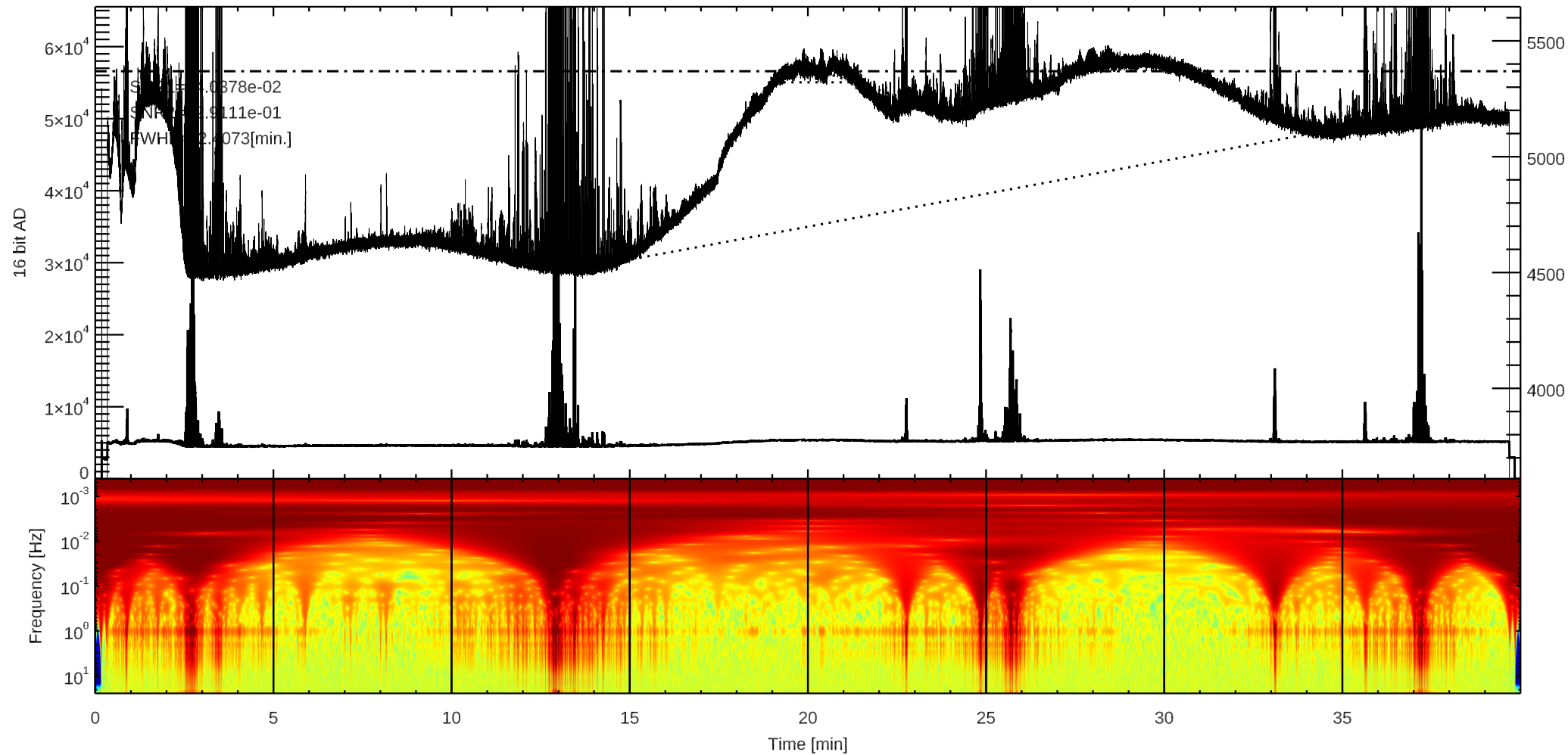
C 3C157 (/home4/archive/swift/dat/2026/10/T20261004045959.dat)
