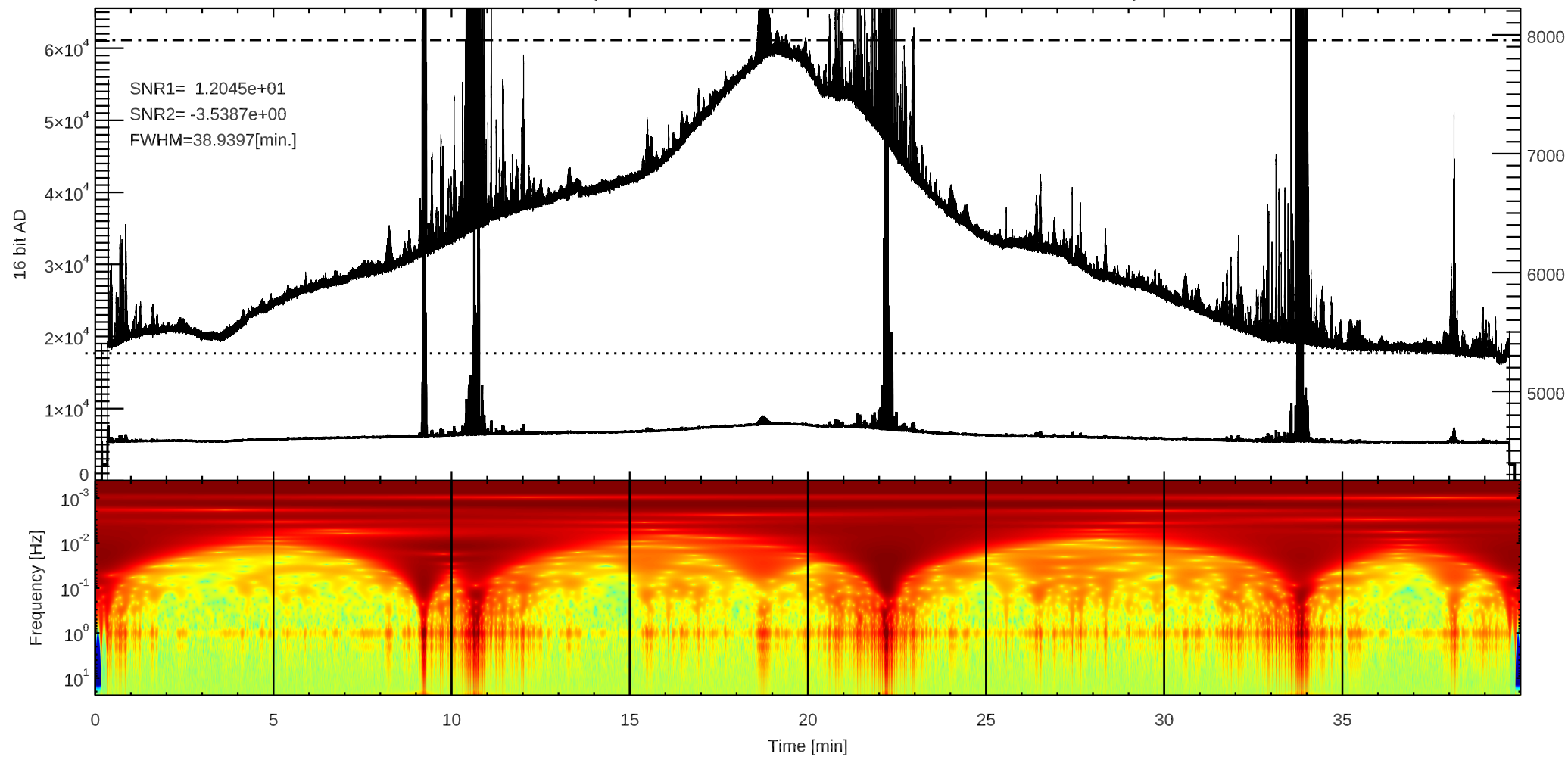
C 3C392 (/home4/archive/swift/dat/2026/10/T20261005173147.dat)
