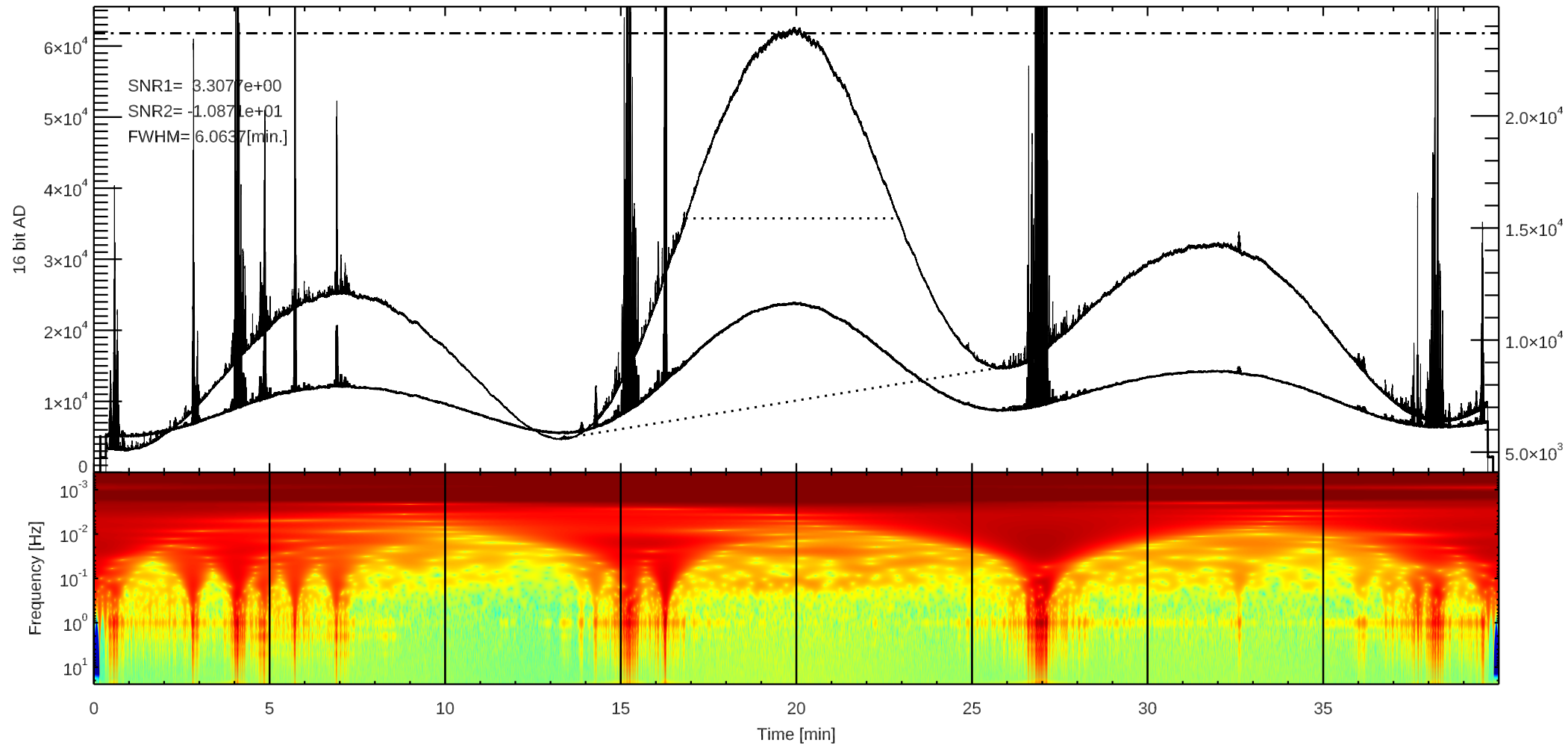
C 3C405 (/home4/archive/swift/dat/2026/10/T20261001185017.dat)
