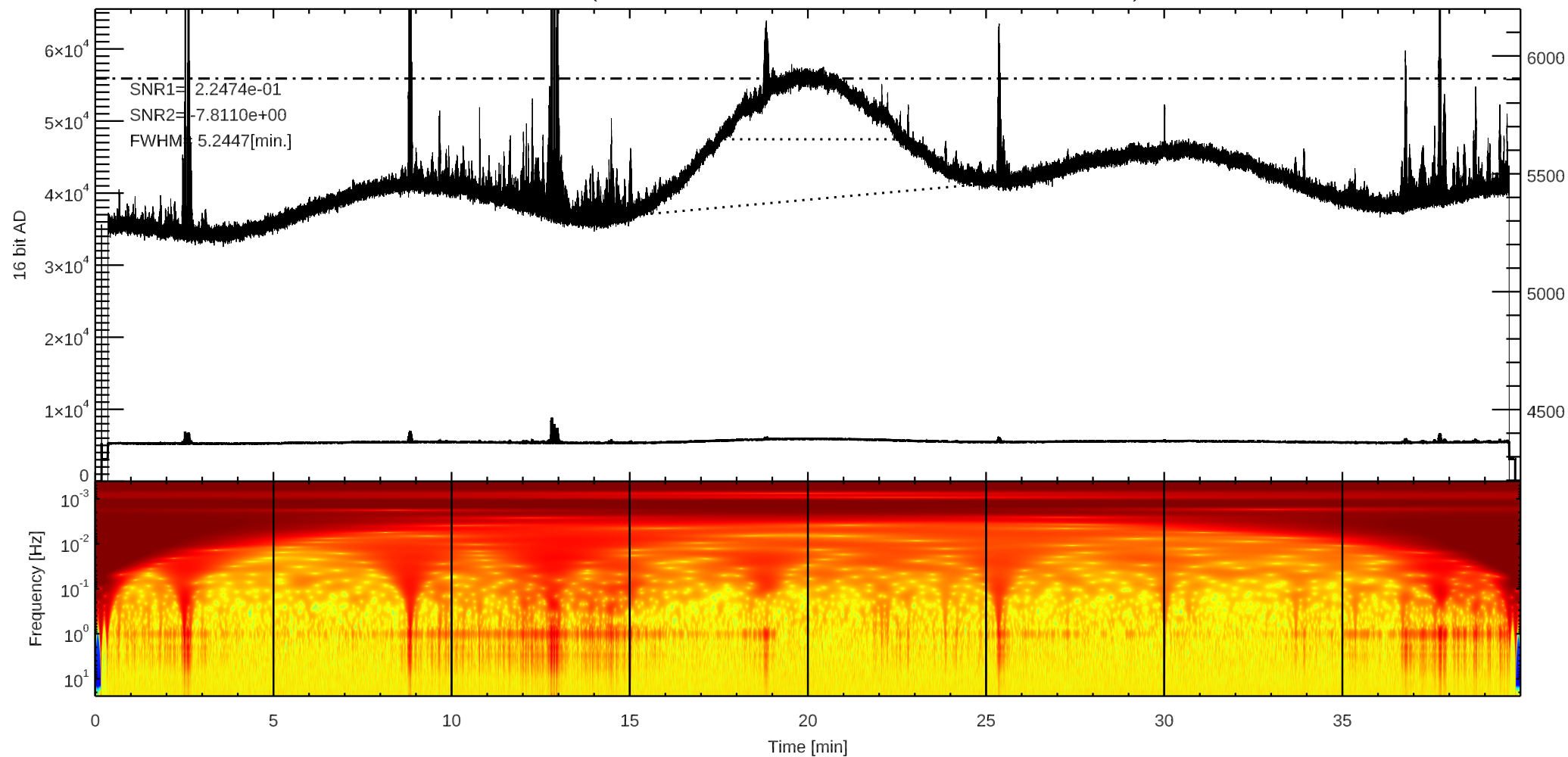
C 3C123 (/home4/archive/swift/dat/2026/10/T20261013024359.dat)
