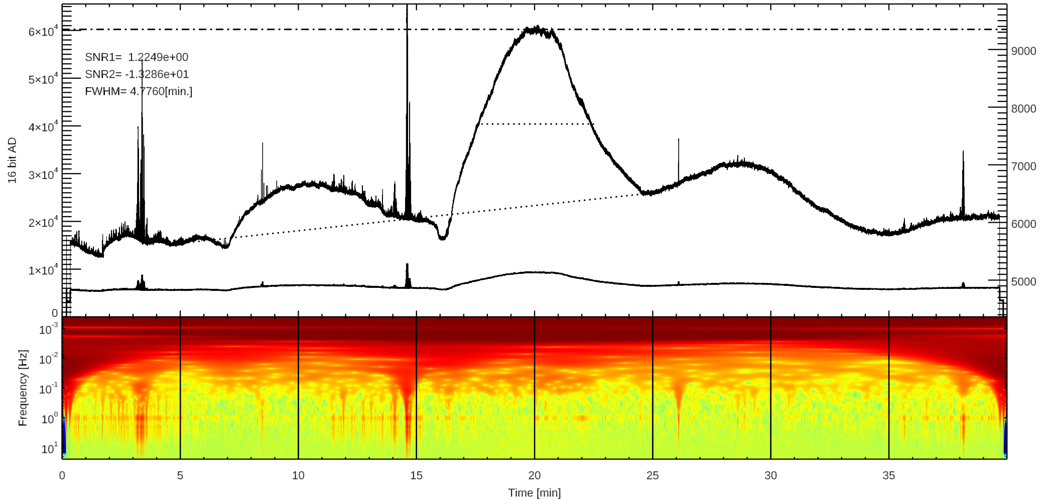
C 3C274 (/home4/archive/swift/dat/2026/05/T20260517202157.dat)
