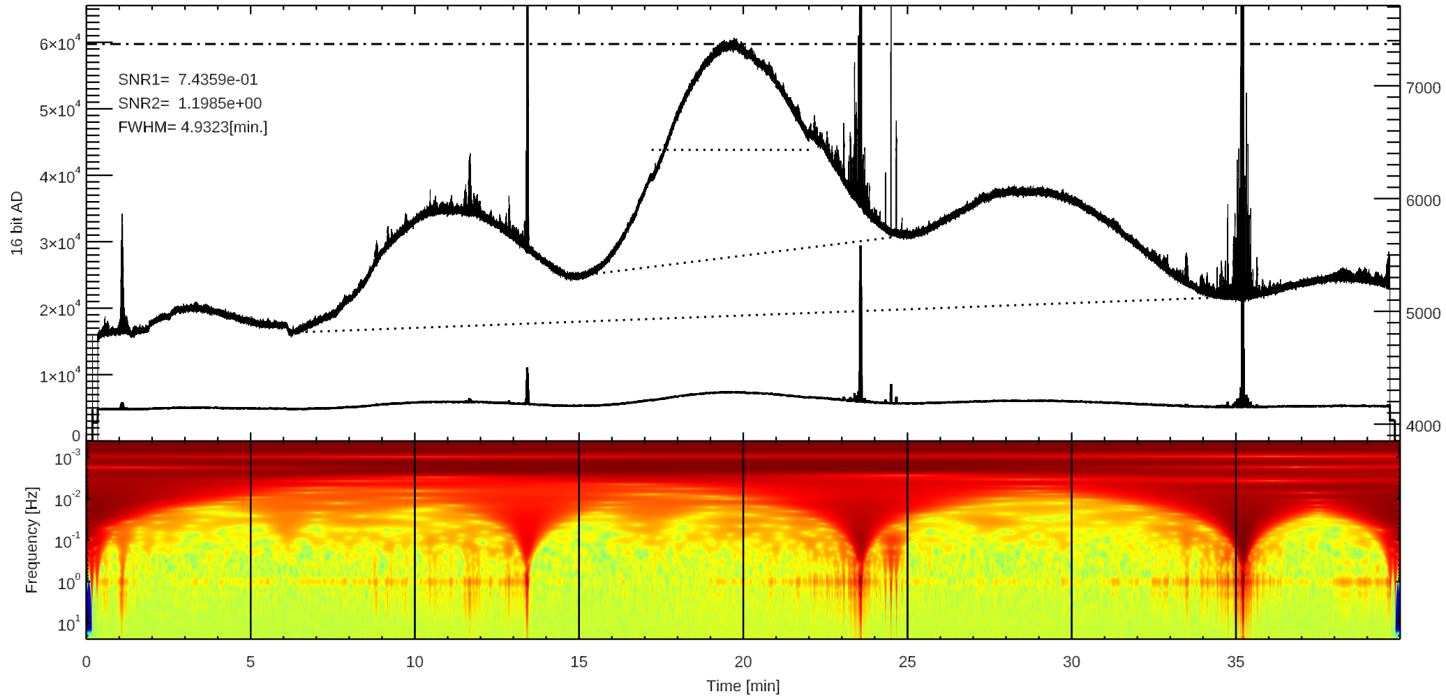
C 3C274 (/home4/archive/swift/dat/2026/05/T20260519201405.dat)
