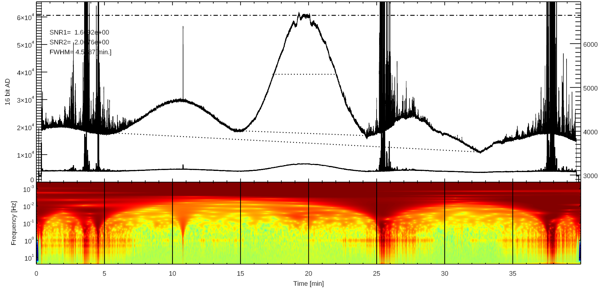
C 3C274 (/home4/archive/swift/dat/2026/05/T20260522200218.dat)
