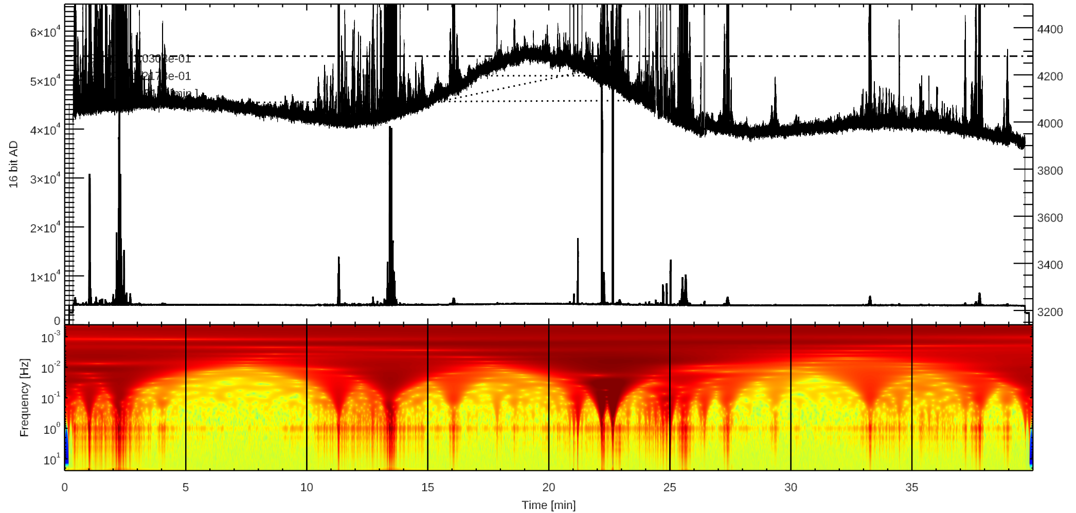
C 3C295 (/home4/archive/swift/dat/2026/05/T20260523213812.dat)
