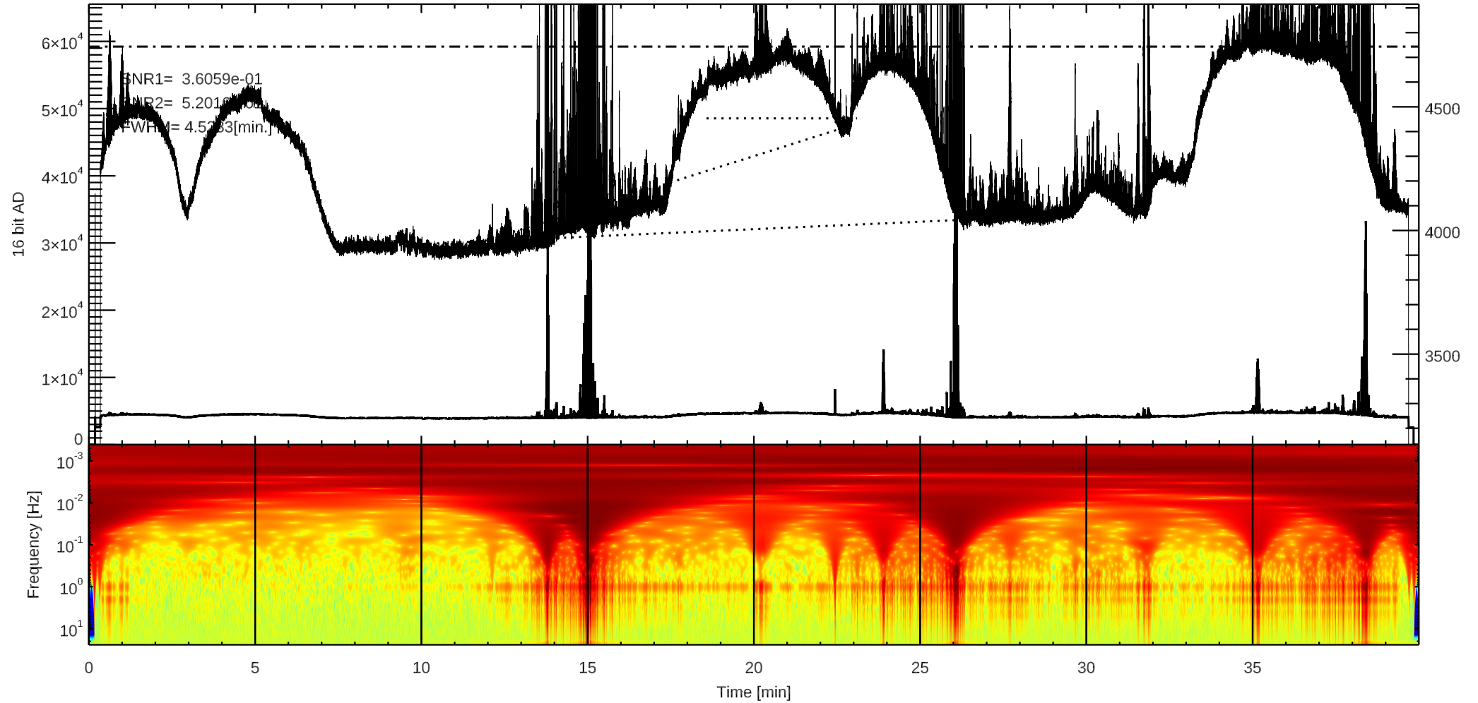
C 3C295 (/home4/archive/swift/dat/2026/06/T20260611202330.dat)
