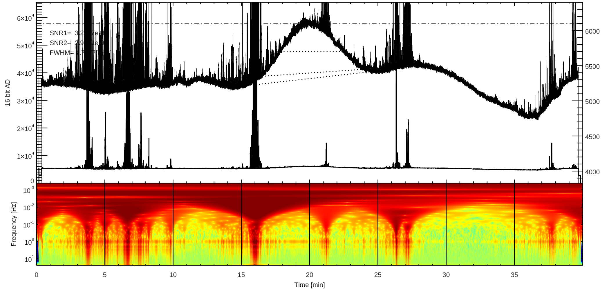
C 3C348 (/home4/archive/swift/dat/2026/05/T20260515005320.dat)
