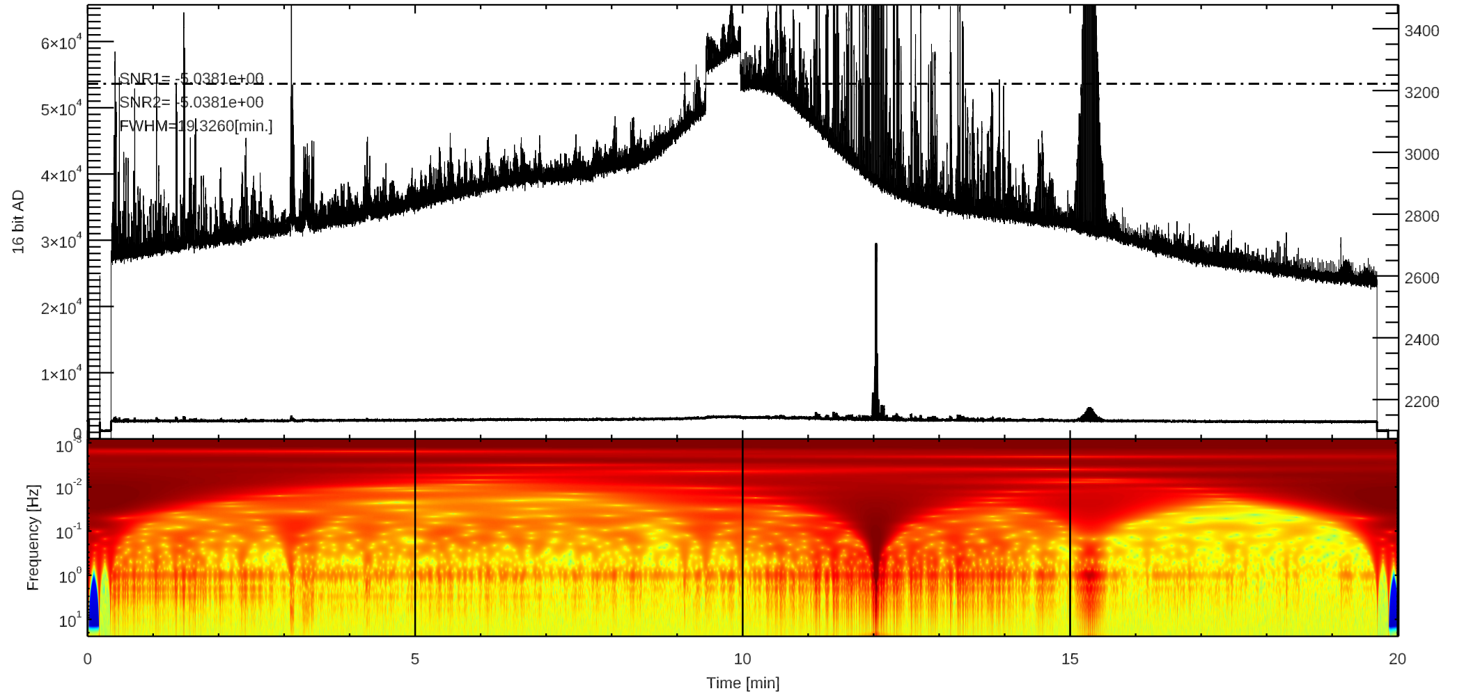
C 3C392 (/home4/archive/fit/dat/2026/08/F20260819204635.dat)
