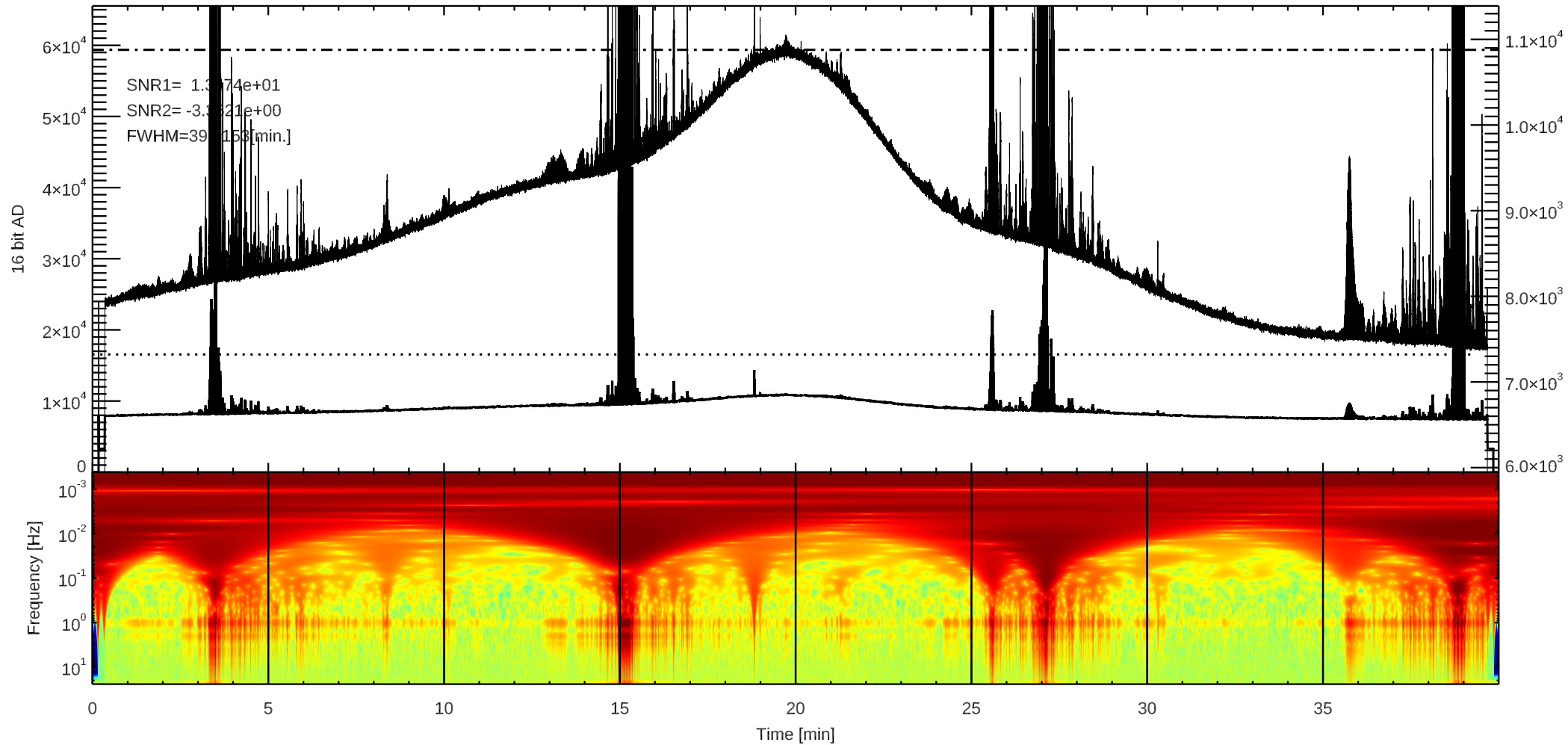
C 3C392 (/home4/archive/swift/dat/2026/05/T20260512030946.dat)
