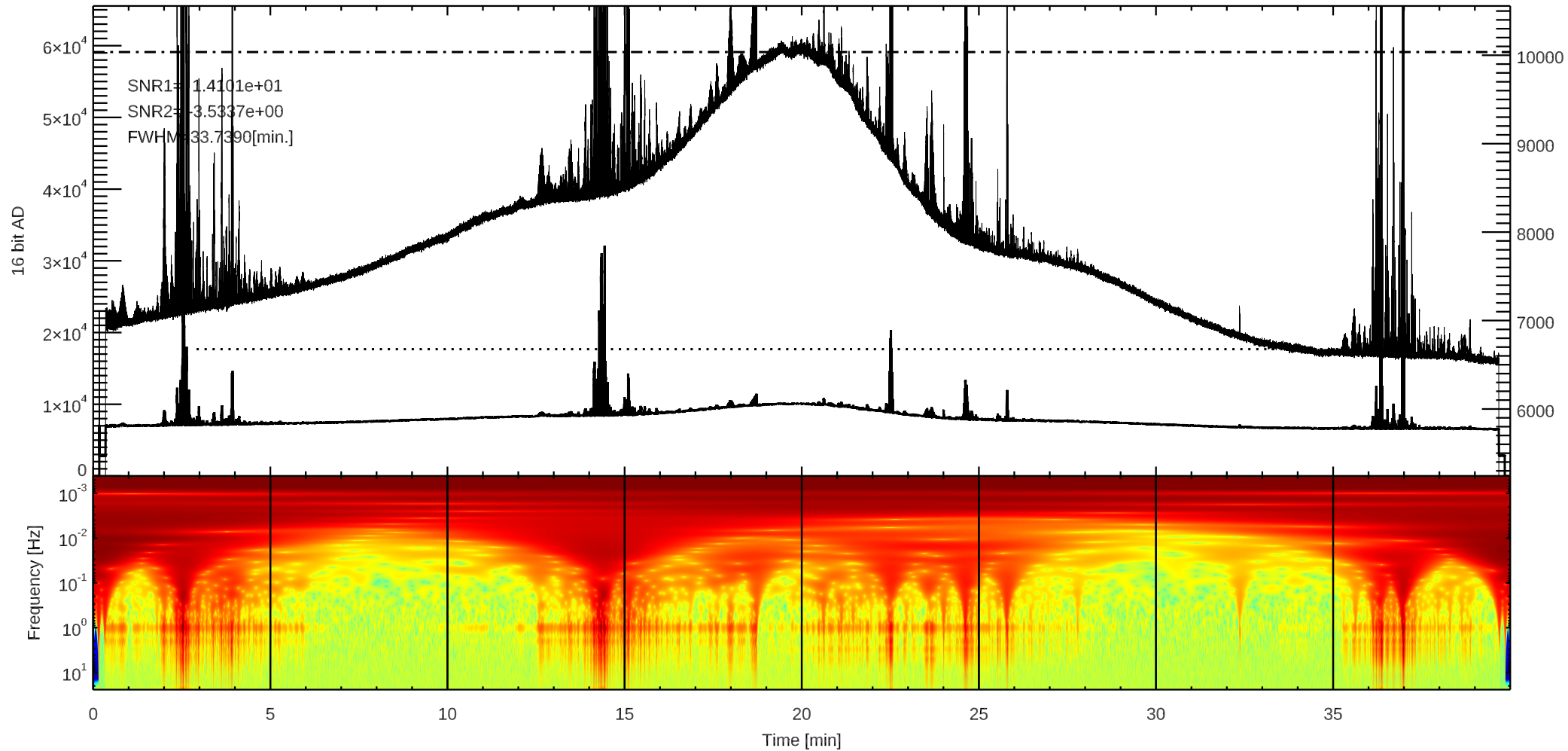
C 3C392 (/home4/archive/swift/dat/2026/06/T20260605013525.dat)
