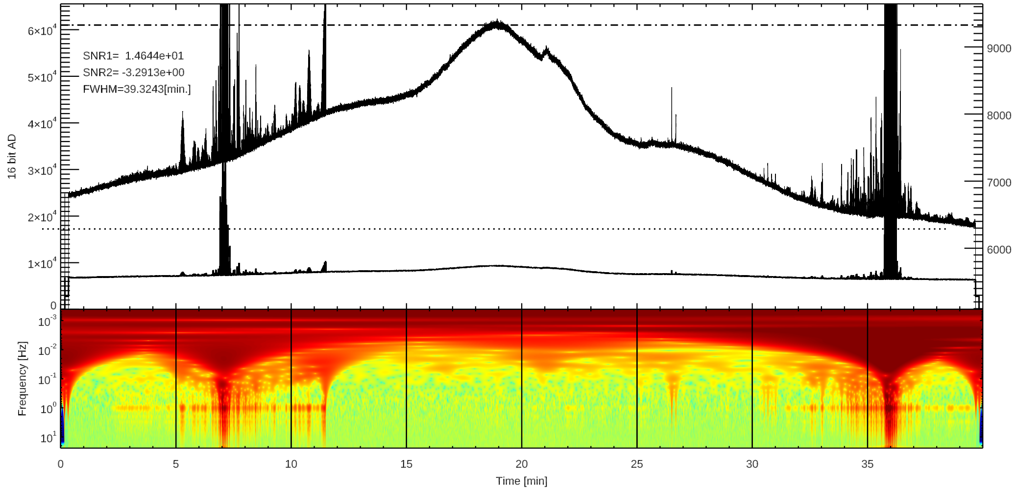
C 3C392 (/home4/archive/swift/dat/2026/06/T20260615005606.dat)
