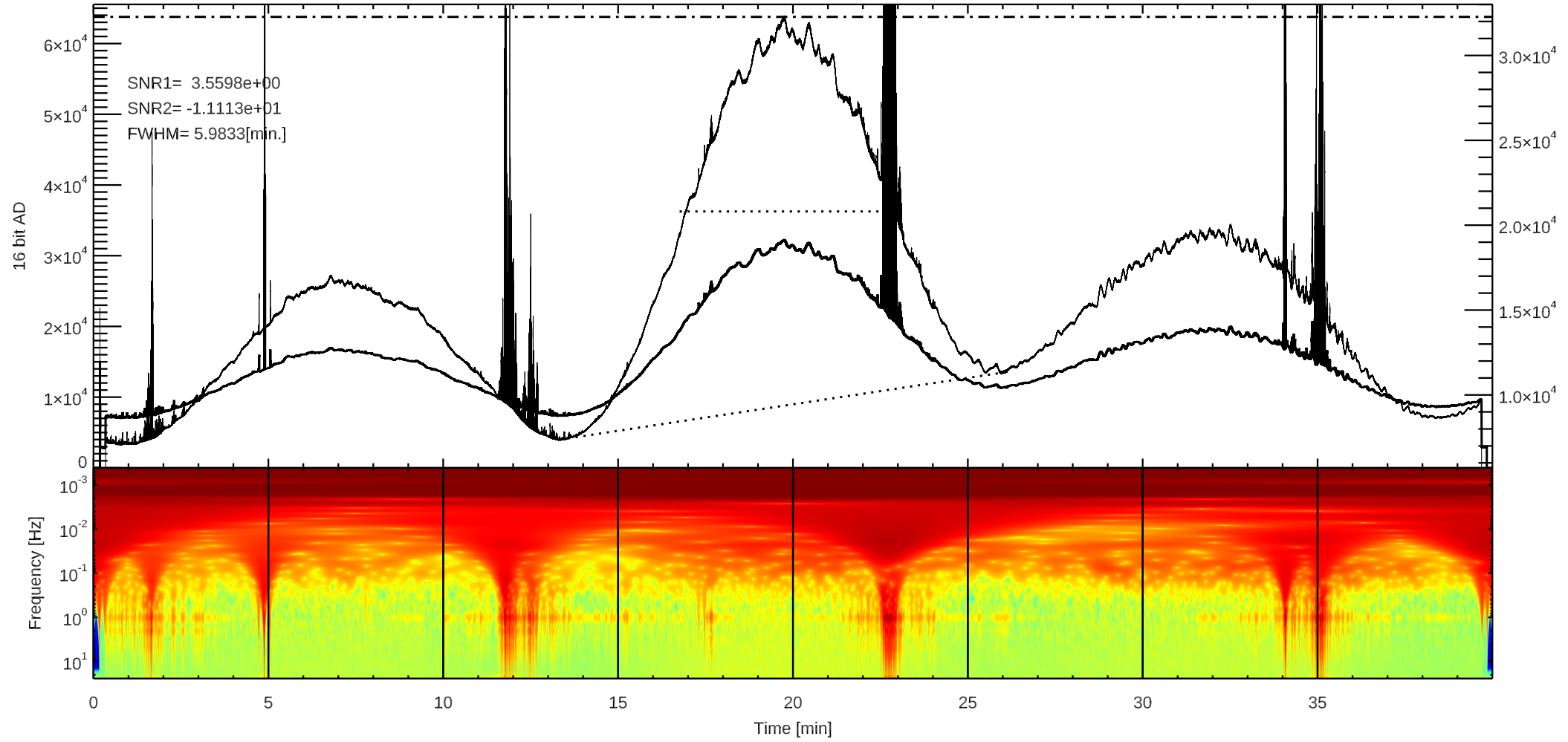
C 3C405 (/home4/archive/swift/dat/2026/05/T20260523032918.dat)
