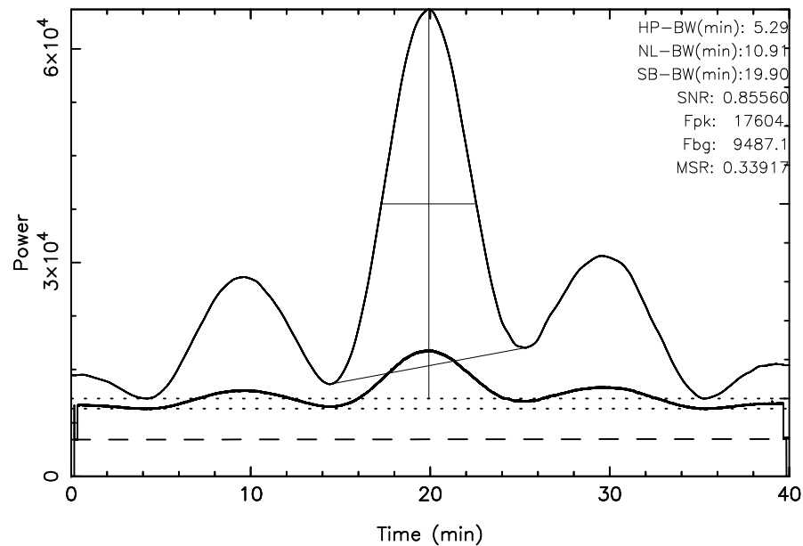
TOYOKAWA 3C144 2024/11/21(326)01:05:50-01:45:50JST
