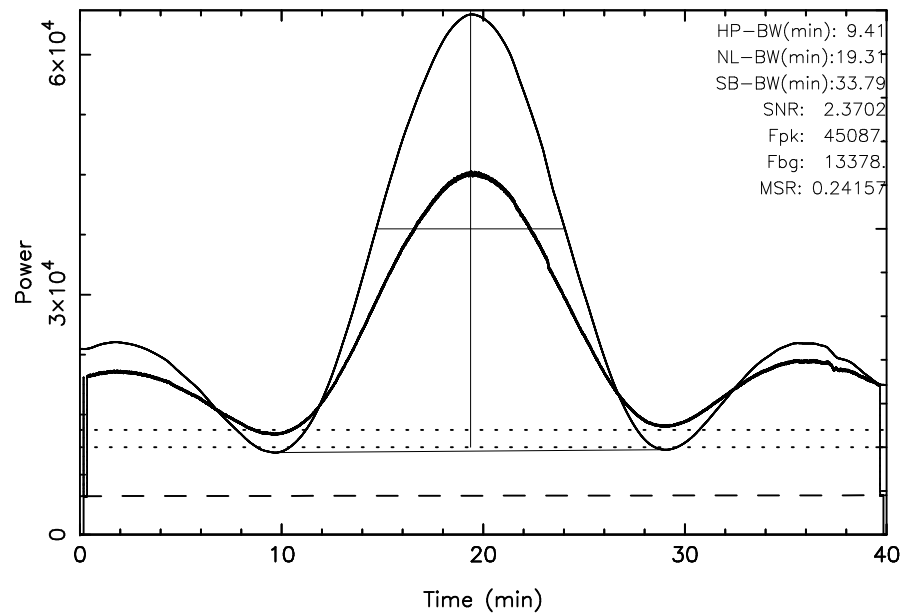
TOYOKAWA 3C461 2024/11/21(326)18:51:24-19:31:24JST
