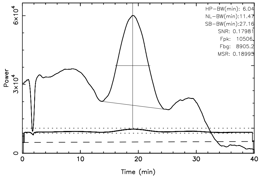
TOYOKAWA 3C157 2024/11/21(326)01:49:14-02:29:14JST
