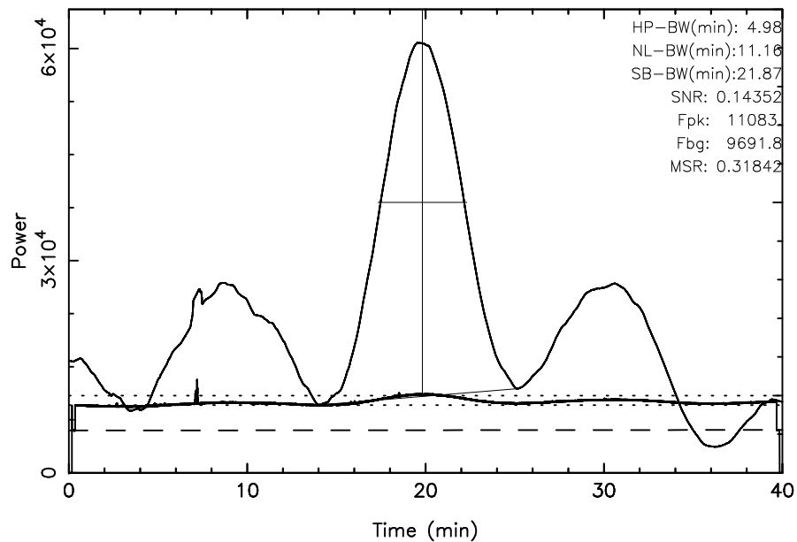
TOYOKAWA 3C123 2024/11/21(326)00:08:37-00:48:37JST
